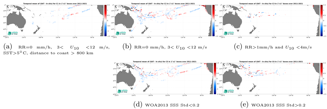
Figure 14: Temporal mean gridded over spatial boxes of size 1^\circ \times 1^\circ of \Delta\text{SSS} (SMOS SSS L4 v2 - Daily (BEC) - TSG (GOSUD-Research-vessel)) for 5 different subdatasets corresponding to:RR=0 mm/h, 3 < U_{10} < 12 m/s, SST>5°C, distance to coast > 800 km (a), RR=0 mm/h, 3 < U_{10} < 12 m/s (b), RR>1mm/h and U_{10} < 4 m/s (c), WOA2013 SSS Std<0.2 (d), WOA2013 SSS Std>0.2 (e).
