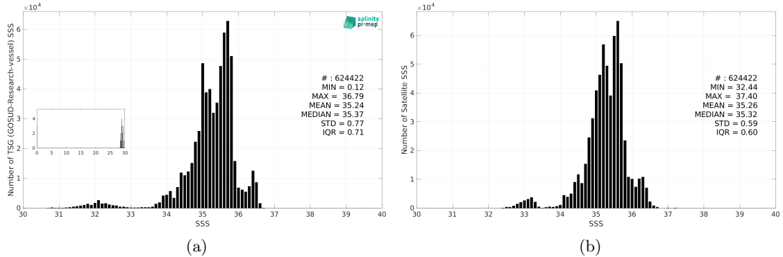
Figure 3: Histograms of SSS from TSG (GOSUD-Research-vessel) (a) and SMOS SSS L4 v2 - Daily (BEC) (b) considering all match-up pairs per bins of 0.1 over the South Pacific Ocean Pi-MEP region and for the full satellite product period.
