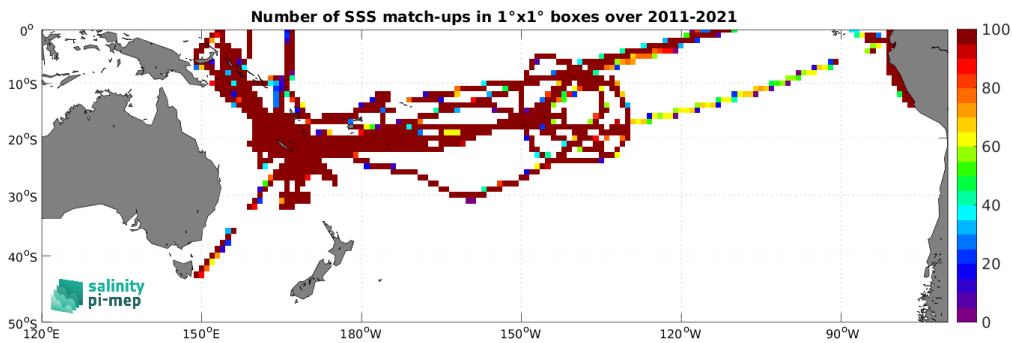
Figure 5: Number of SSS match-ups between TSG (GOSUD-Research-vessel) SSS and the SMOS SSS L4 v2 - Daily (BEC) SSS product for the South Pacific Ocean Pi-MEP region over 1^\circ \times 1^\circ boxes and for the full satellite product period.
