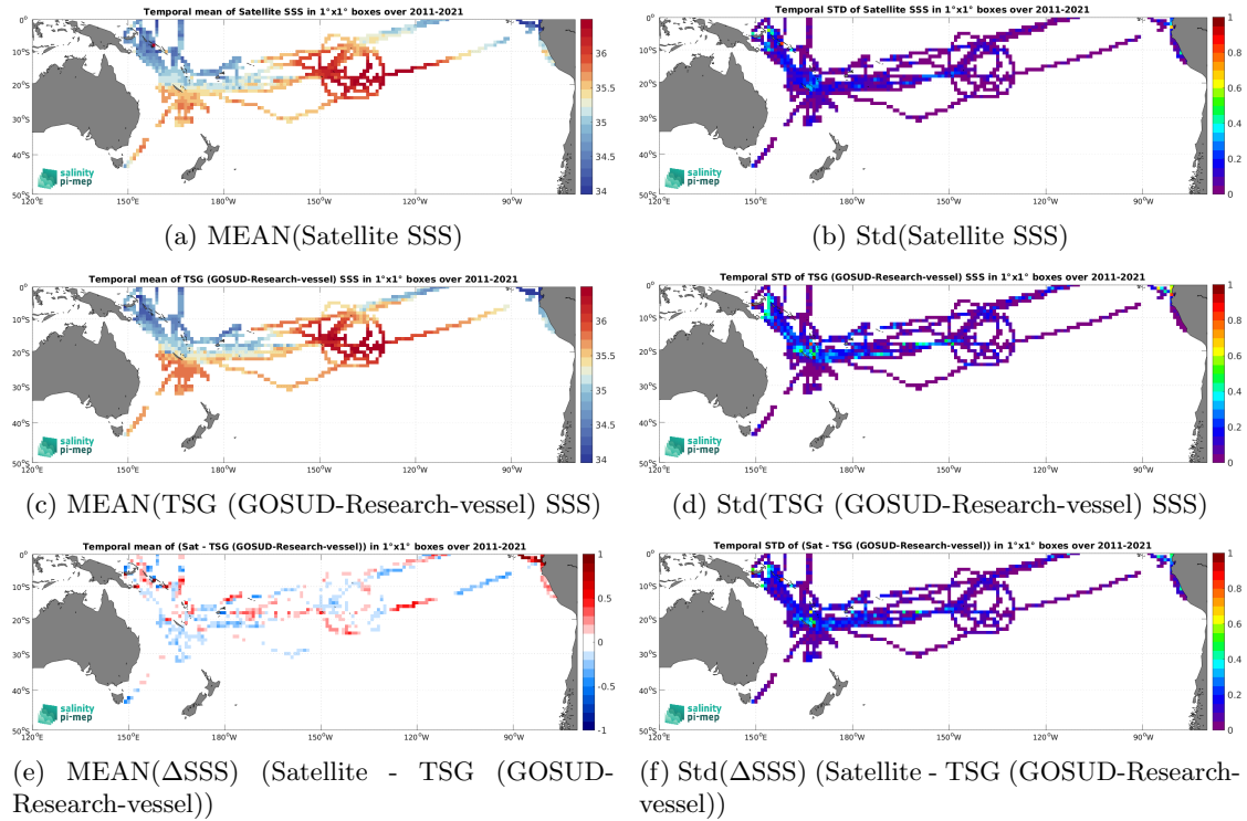
Figure 7: Temporal mean (left) and Std (right) of SSS from SMOS SSS L4 v2 - Daily (BEC) (top), TSG (GOSUD-Research-vessel) (middle), and of \Delta SSS (Satellite - TSG (GOSUD-Research-vessel)). Only match-up pairs are used to generate these maps.
