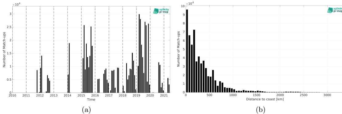
Figure 2: Number of match-ups between TSG (GOSUD-Research-vessel) and SMOS SSS L4 v2 - Daily (BEC) SSS as a function of time (a) and as function of the distance to coast (b) over the South Pacific Ocean Pi-MEP region and for the full satellite product period.
