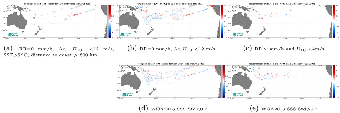
Figure 12: Temporal mean gridded over spatial boxes of size 1^\circ \times 1^\circ of \Delta\text{SSS} (SMOS SSS L4 v2 - Daily (BEC) - TSG (GOSUD-Research-vessel)) for 5 different subdatasets corresponding to:RR=0 mm/h, 3 < U_{10} < 12 m/s, SST >5^\circ\text{C} , distance to coast > 800 km (a), RR=0 mm/h, 3 < U_{10} < 12 m/s (b), RR >1 mm/h and U_{10} < 4 m/s (c), WOA2013 SSS Std <0.2 (d), WOA2013 SSS Std >0.2 (e).
