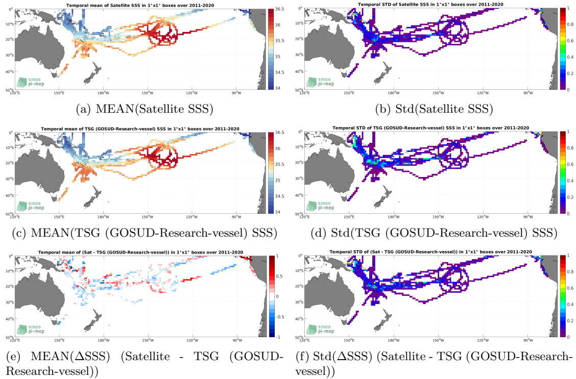
Figure 6: Temporal mean (left) and Std (right) of SSS from SMOS SSS L4 v2 - Daily (BEC) (top), TSG (GOSUD-Research-vessel) (middle), and of \Delta SSS (Satellite - TSG (GOSUD-Research-vessel)). Only match-up pairs are used to generate these maps.
