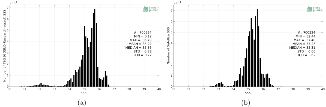
Figure 2: Histograms of SSS from TSG (GOSUD-Research-vessel) (a) and SMOS SSS L4 v2 - Daily (BEC) (b) considering all match-up pairs per bins of 0.1 over the South Pacific Ocean Pi-MEP region and for the full satellite product period.
