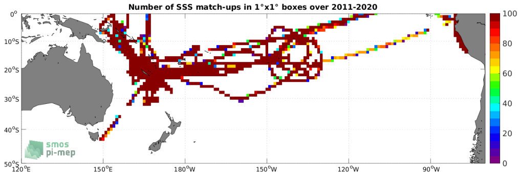
Figure 4: Number of SSS match-ups between TSG (GOSUD-Research-vessel) SSS and the SMOS SSS L4 v2 - Daily (BEC) SSS product for the South Pacific Ocean Pi-MEP region over 1^\circ \times 1^\circ boxes and for the full satellite product period.
