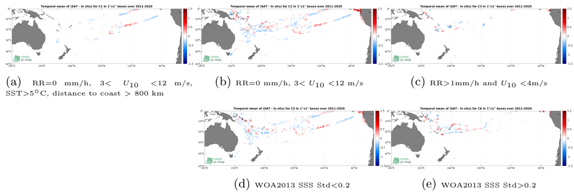
Figure 12: Temporal mean gridded over spatial boxes of size 1^\circ \times 1^\circ of \Delta SSS (SMOS SSS L4 v2 - Daily (BEC) - TSG (GOSUD-Research-vessel)) for 5 different subdatasets corresponding to:RR=0 mm/h, 3 < U_{10} < 12 m/s, SST >5^\circ C, distance to coast > 800 km (a), RR=0 mm/h, 3 < U_{10} < 12 m/s (b), RR >1 mm/h and U_{10} < 4 m/s (c), WOA2013 SSS Std <0.2 (d), WOA2013 SSS Std >0.2 (e).
