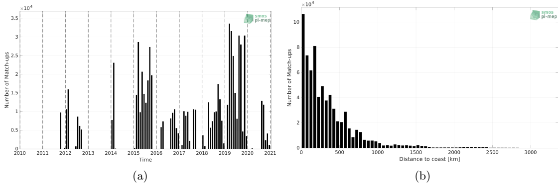
Figure 1: Number of match-ups between TSG (GOSUD-Research-vessel) and SMOS SSS L4 v2 - Daily (BEC) SSS as a function of time (a) and as function of the distance to coast (b) over the South Pacific Ocean Pi-MEP region and for the full satellite product period.
