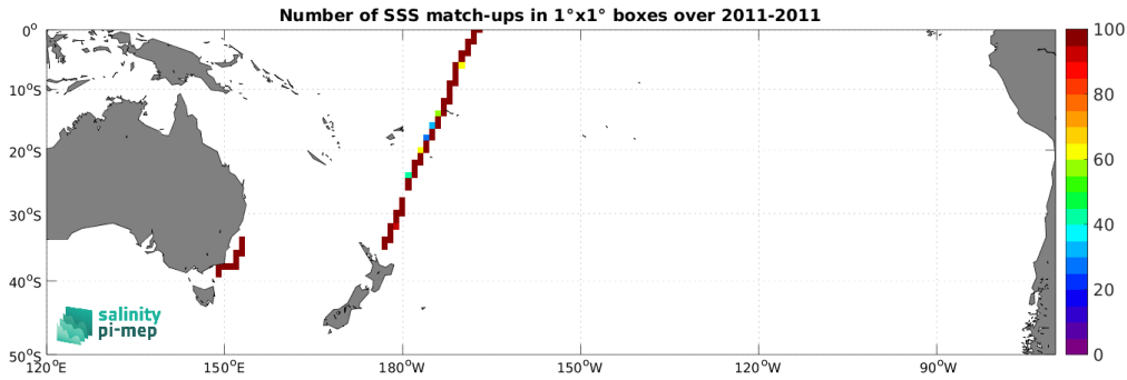
Figure 5: Number of SSS match-ups between TSG (CSIC-UTM) SSS and the SMOS SSS L4 v2 - Daily (BEC) SSS product for the South Pacific Ocean Pi-MEP region over 1^\circ \times 1^\circ boxes and for the full satellite product period.
