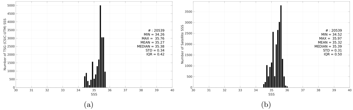
Figure 3: Histograms of SSS from TSG (CSIC-UTM) (a) and SMOS SSS L4 v2 - Daily (BEC) (b) considering all match-up pairs per bins of 0.1 over the South Pacific Ocean Pi-MEP region and for the full satellite product period.
