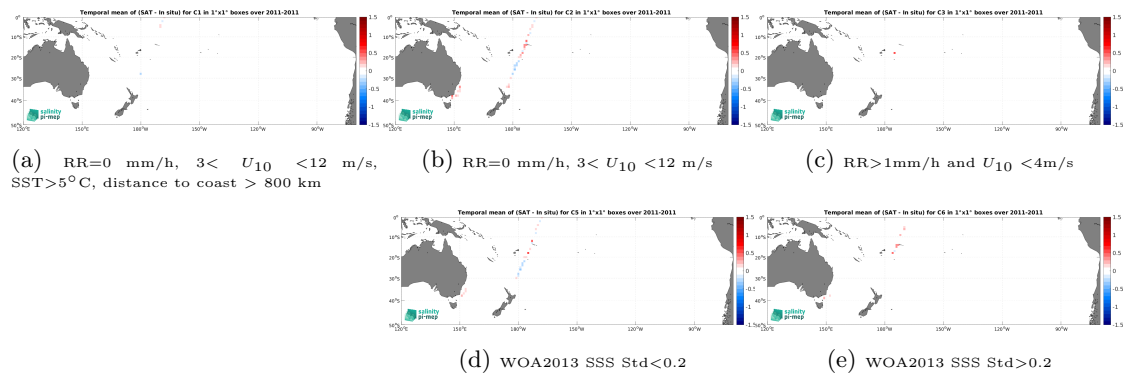
Figure 14: Temporal mean gridded over spatial boxes of size 1^\circ \times 1^\circ of \Delta\text{SSS} (SMOS SSS L4 v2 - Daily (BEC) - TSG (CSIC-UTM)) for 5 different subdatasets corresponding to:RR=0 mm/h, 3 < U_{10} < 12 m/s, SST>5°C, distance to coast > 800 km (a), RR=0 mm/h, 3 < U_{10} < 12 m/s (b), RR>1mm/h and U_{10} < 4 m/s (c), WOA2013 SSS Std<0.2 (d), WOA2013 SSS Std>0.2 (e).
