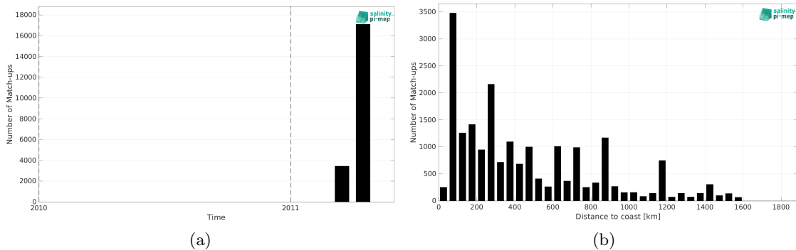
Figure 2: Number of match-ups between TSG (CSIC-UTM) and SMOS SSS L4 v2 - Daily (BEC) SSS as a function of time (a) and as function of the distance to coast (b) over the South Pacific Ocean Pi-MEP region and for the full satellite product period.
