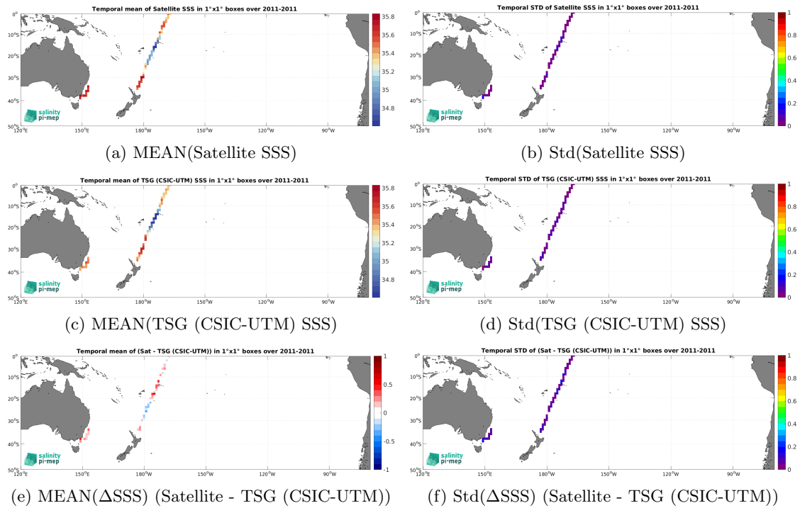
Figure 7: Temporal mean (left) and Std (right) of SSS from SMOS SSS L4 v2 - Daily (BEC) (top), TSG (CSIC-UTM) (middle), and of \Delta SSS (Satellite - TSG (CSIC-UTM)). Only match-up pairs are used to generate these maps.
