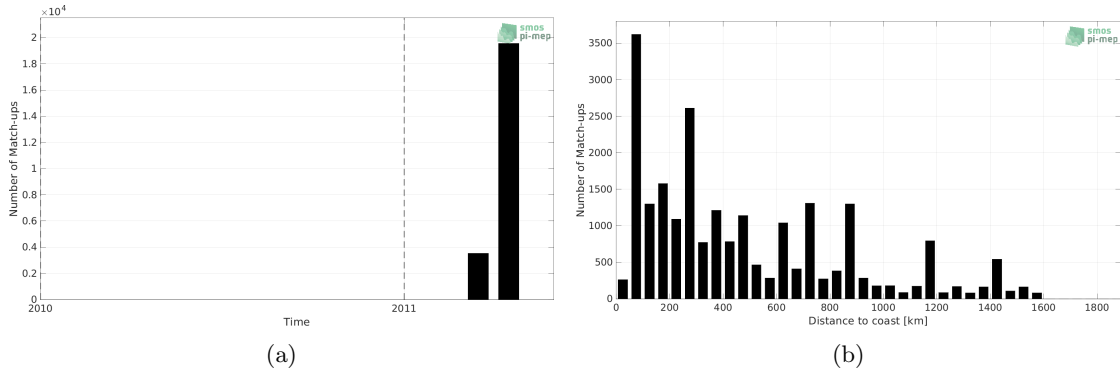
Figure 1: Number of match-ups between TSG (CSIC-UTM) and SMOS SSS L4 v2 - Daily (BEC) SSS as a function of time (a) and as function of the distance to coast (b) over the South Pacific Ocean Pi-MEP region and for the full satellite product period.
