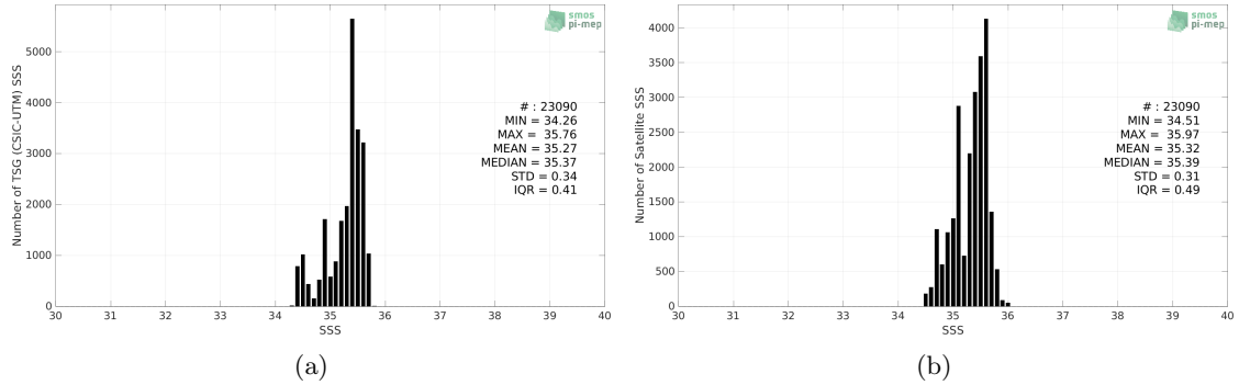
Figure 2: Histograms of SSS from TSG (CSIC-UTM) (a) and SMOS SSS L4 v2 - Daily (BEC) (b) considering all match-up pairs per bins of 0.1 over the South Pacific Ocean Pi-MEP region and for the full satellite product period.
