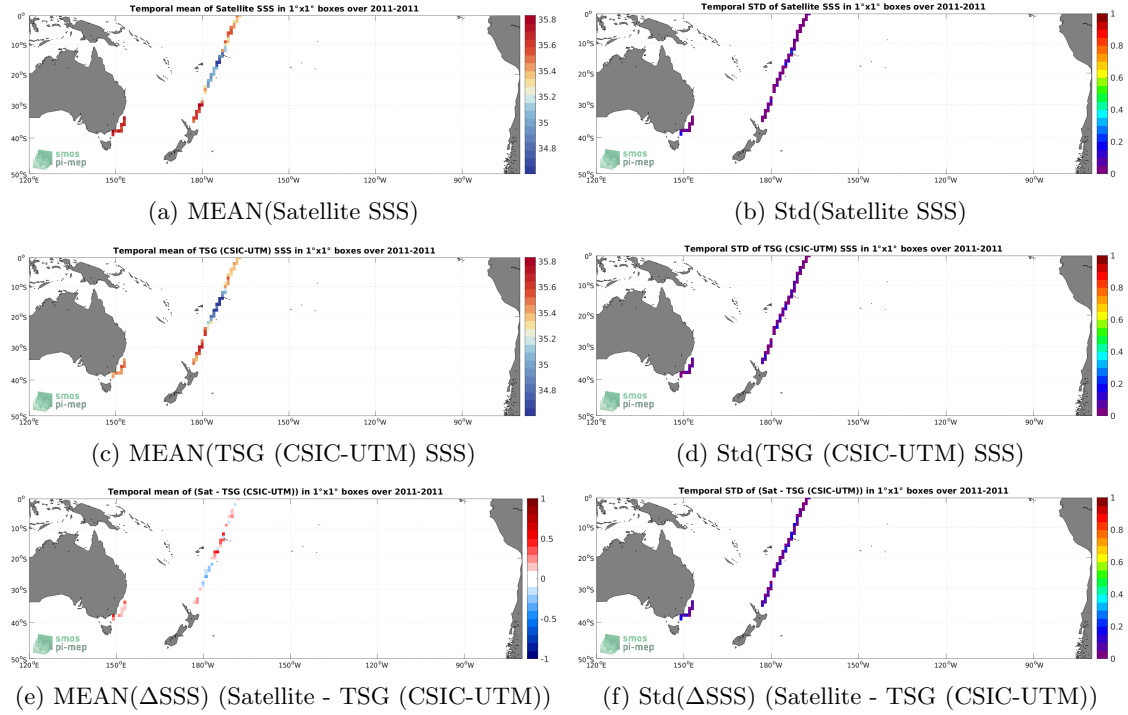
Figure 6: Temporal mean (left) and Std (right) of SSS from SMOS SSS L4 v2 - Daily (BEC) (top), TSG (CSIC-UTM) (middle), and of \Delta SSS (Satellite - TSG (CSIC-UTM)). Only match-up pairs are used to generate these maps.
