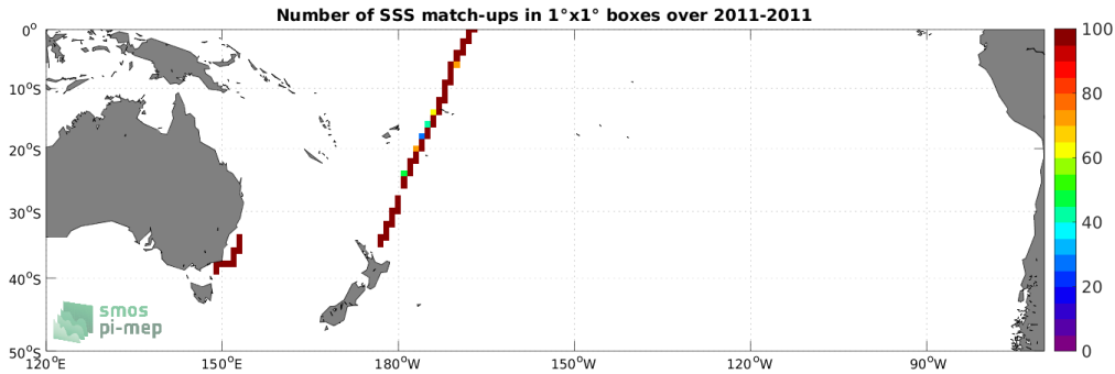
Figure 4: Number of SSS match-ups between TSG (CSIC-UTM) SSS and the SMOS SSS L4 v2 - Daily (BEC) SSS product for the South Pacific Ocean Pi-MEP region over 1^\circ \times 1^\circ boxes and for the full satellite product period.
