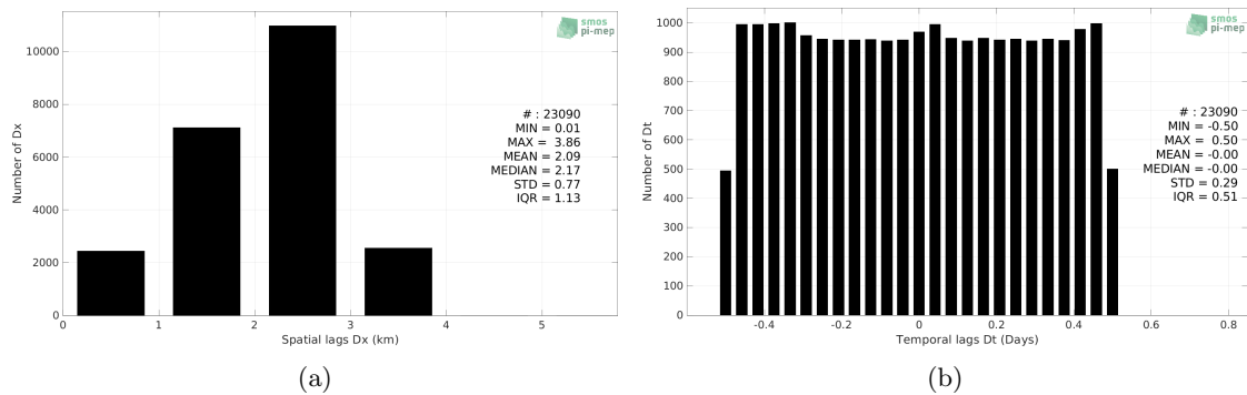
Figure 5: Histograms of the spatial (a) and temporal (b) lags between the location/time of the TSG (CSIC-UTM) measurement and the date of the corresponding SMOS SSS L4 v2 - Daily (BEC) SSS pixel.
