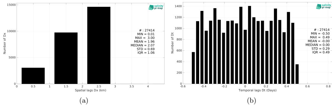
Figure 6: Histograms of the spatial (a) and temporal (b) lags between the location/time of the Saildrone measurement and the date of the corresponding SMOS SSS L4 v2 - Daily (BEC) SSS pixel.
