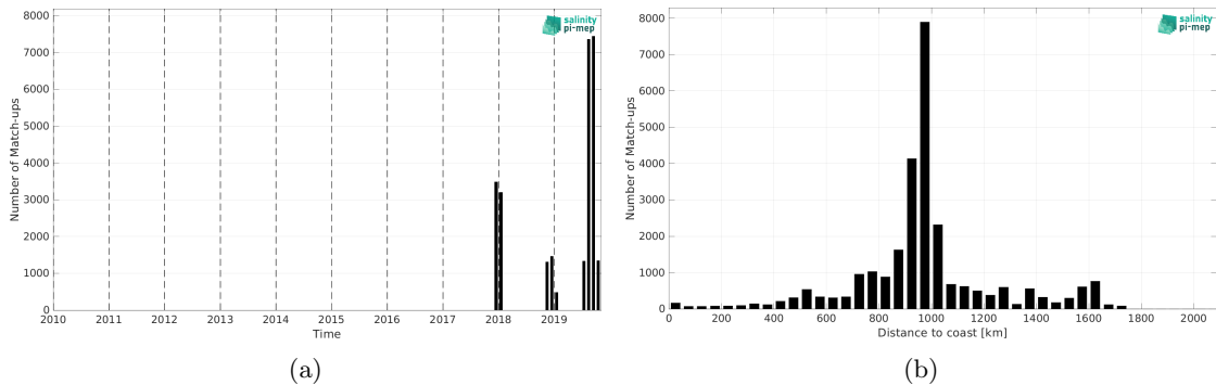
Figure 2: Number of match-ups between Saildrone and SMOS SSS L4 v2 - Daily (BEC) SSS as a function of time (a) and as function of the distance to coast (b) over the South Pacific Ocean Pi-MEP region and for the full satellite product period.
