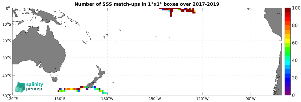
Figure 5: Number of SSS match-ups between Saildrone SSS and the SMOS SSS L4 v2 - Daily (BEC) SSS product for the South Pacific Ocean Pi-MEP region over 1^\circ \times 1^\circ boxes and for the full satellite product period.
