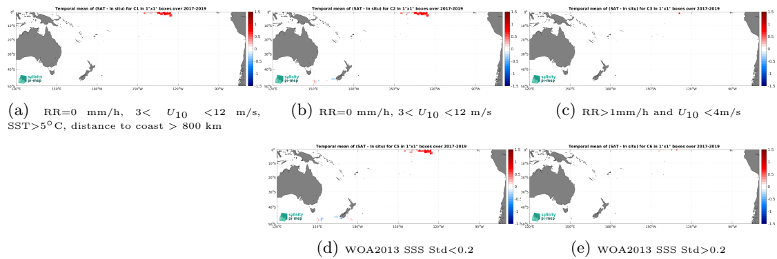
Figure 14: Temporal mean gridded over spatial boxes of size 1^\circ \times 1^\circ of \Delta\text{SSS} (SMOS SSS L4 v2 - Daily (BEC) - Saildrone) for 5 different subdatasets corresponding to:RR=0 mm/h, 3 < U_{10} < 12 m/s, SST>5°C, distance to coast > 800 km (a), RR=0 mm/h, 3 < U_{10} < 12 m/s (b), RR>1mm/h and U_{10} < 4 m/s (c), WOA2013 SSS Std<0.2 (d), WOA2013 SSS Std>0.2 (e).
