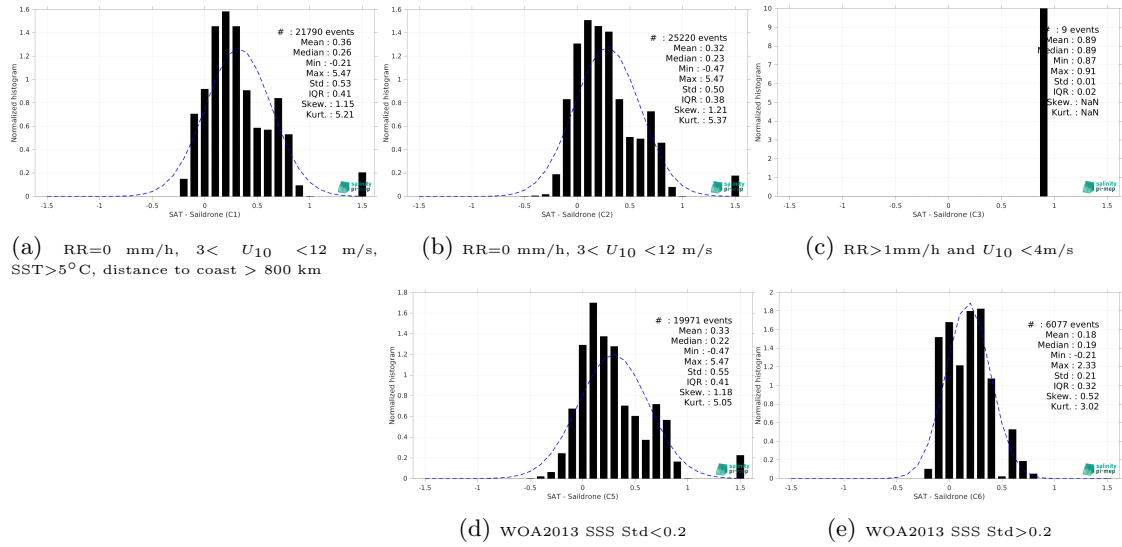
Figure 15: Normalized histogram of \Delta SSS (SMOS SSS L4 v2 - Daily (BEC) - Saildrone) for 5 different subdatasets corresponding to: RR=0 mm/h, 3 < U_{10} < 12 m/s, SST > 5°C, distance to coast > 800 km (a), RR=0 mm/h, 3 < U_{10} < 12 m/s (b), RR > 1mm/h and U_{10} < 4 m/s (c), WOA2013 SSS Std < 0.2 (d), WOA2013 SSS Std > 0.2 (e).
