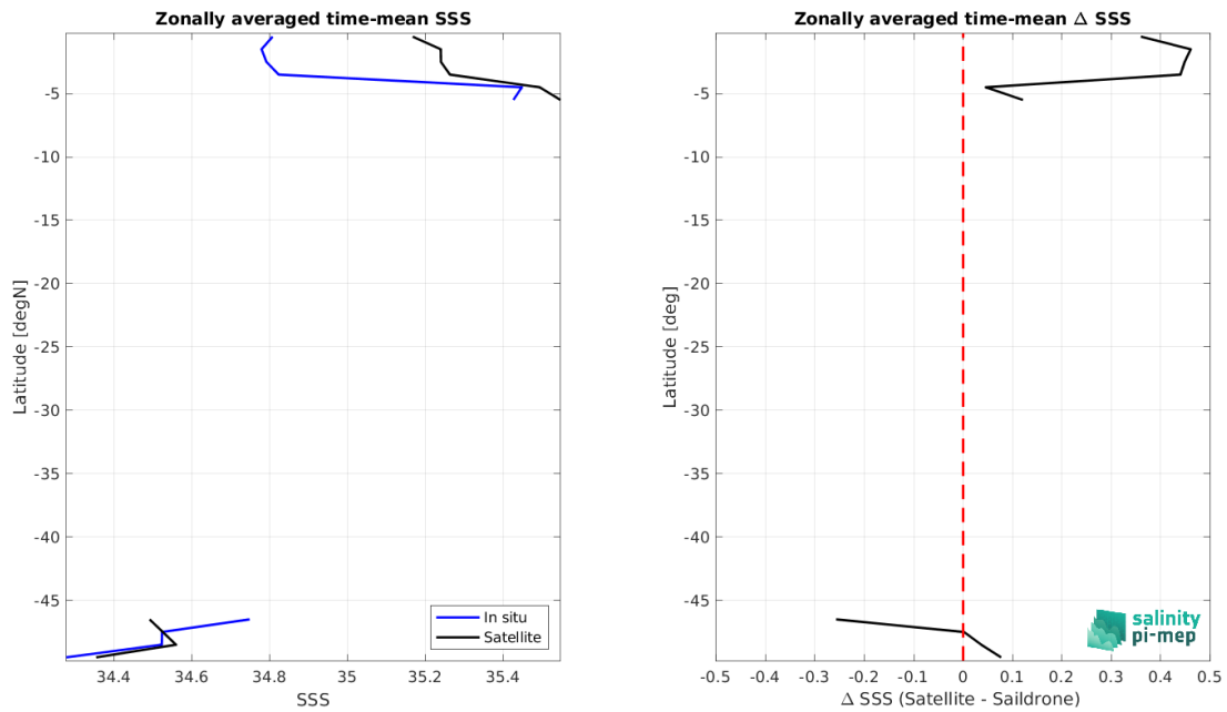
Figure 9: Left panel: Zonal mean SSS from SMOS SSS L4 v2 - Daily (BEC) satellite product (black) and from Saildrone (blue). Right panel: Zonal mean of \Delta SSS (Satellite - Saildrone) for all the collected Pi-MEP match-up pairs estimated over the full satellite product period.
