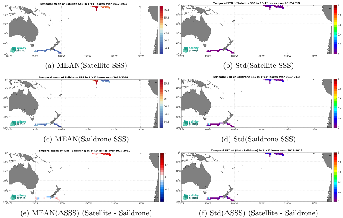
Figure 7: Temporal mean (left) and Std (right) of SSS from SMOS SSS L4 v2 - Daily (BEC) (top), Saildrone (middle), and of \Delta SSS (Satellite - Saildrone). Only match-up pairs are used to generate these maps.
