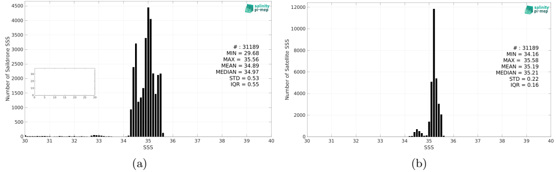
Figure 2: Histograms of SSS from Saildrone (a) and SMOS SSS L4 v2 - Daily (BEC) (b) considering all match-up pairs per bins of 0.1 over the South Pacific Ocean Pi-MEP region and for the full satellite product period.
