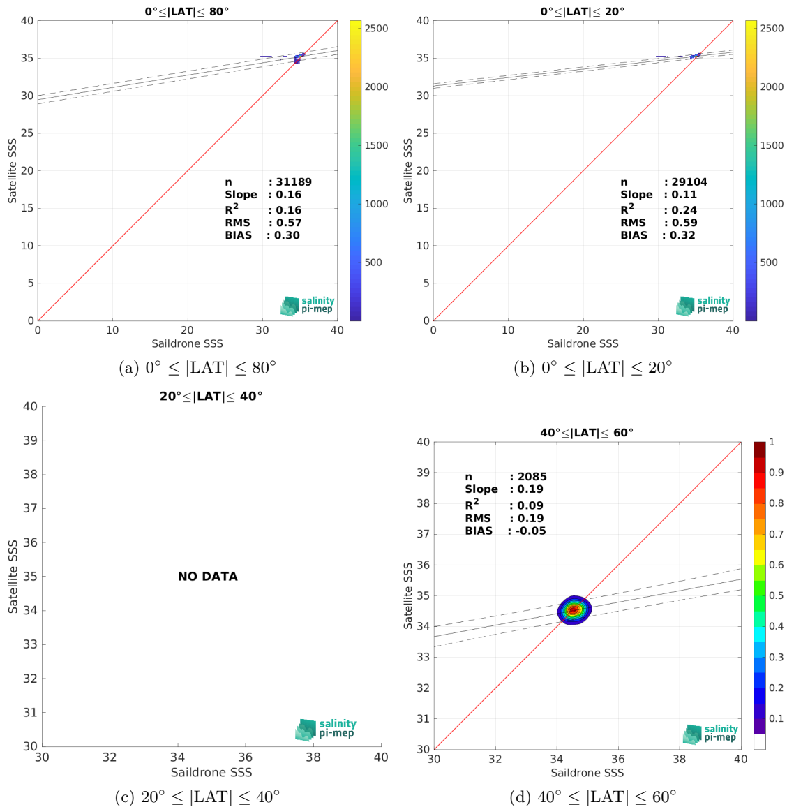
Figure 9: Contour maps of the concentration of SMOS SSS L4 v2 - Daily (BEC) SSS (y-axis) versus Sairdrone SSS (x-axis) at match-up pairs for different latitude bands. For each plot, the red line shows x=y . The black thin and dashed lines indicate a linear fit through the data cloud and the \pm 95\% confidence levels, respectively. The number match-up pairs n , the slope and R^2 coefficient of the linear fit, the root mean square (RMS) and the mean bias between satellite and in situ data are indicated for each latitude band in each plots.
