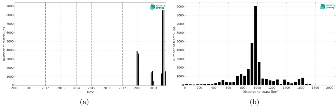
Figure 1: Number of match-ups between Saildrone and SMOS SSS L4 v2 - Daily (BEC) SSS as a function of time (a) and as function of the distance to coast (b) over the South Pacific Ocean Pi-MEP region and for the full satellite product period.
