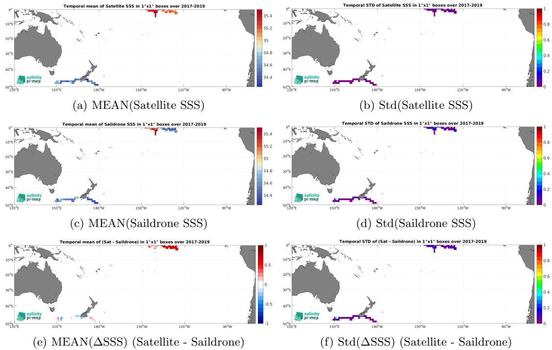
Figure 6: Temporal mean (left) and Std (right) of SSS from SMOS SSS L4 v2 - Daily (BEC) (top), Saildrone (middle), and of \Delta SSS (Satellite - Saildrone). Only match-up pairs are used to generate these maps.
