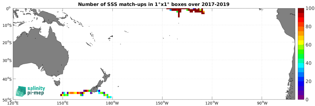
Figure 4: Number of SSS match-ups between Saildrone SSS and the SMOS SSS L4 v2 - Daily (BEC) SSS product for the South Pacific Ocean Pi-MEP region over 1^\circ \times 1^\circ boxes and for the full satellite product period.
