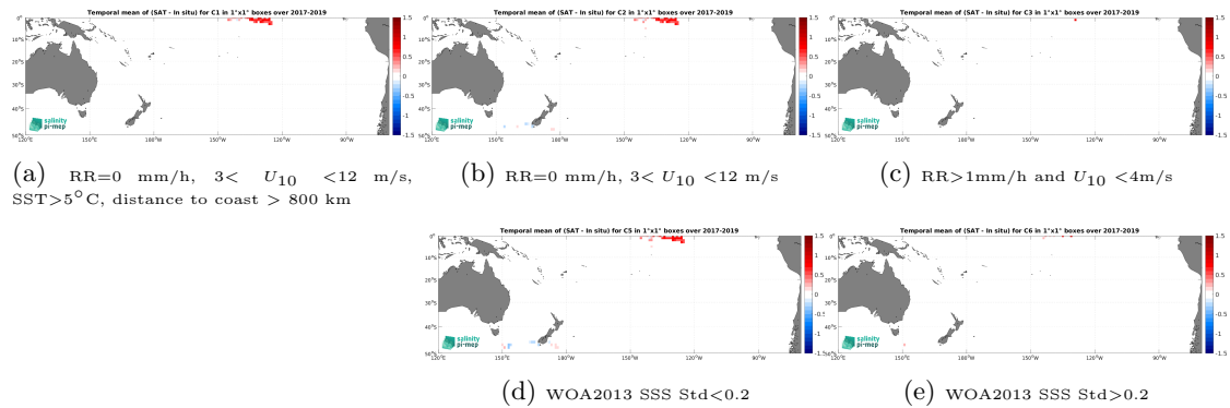
Figure 12: Temporal mean gridded over spatial boxes of size 1^\circ \times 1^\circ of \Delta SSS (SMOS SSS L4 v2 - Daily (BEC) - Saikrone) for 5 different subdatasets corresponding to:RR=0 mm/h, 3 < U_{10} < 12 m/s, SST >5^\circ\text{C} , distance to coast > 800 km (a), RR=0 mm/h, 3 < U_{10} < 12 m/s (b), RR >1 mm/h and U_{10} < 4 m/s (c), WOA2013 SSS Std <0.2 (d), WOA2013 SSS Std >0.2 (e).
