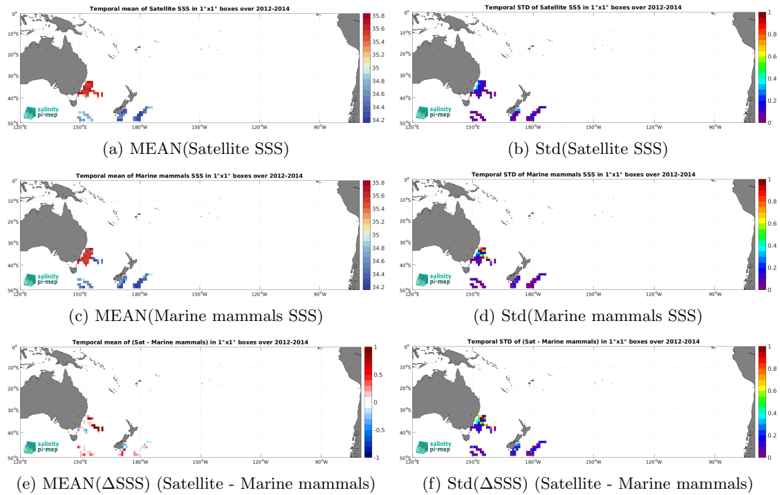
Figure 7: Temporal mean (left) and Std (right) of SSS from SMOS SSS L4 v2 - Daily (BEC) (top), Marine mammals (middle), and of \Delta SSS (Satellite - Marine mammals). Only match-up pairs are used to generate these maps.
