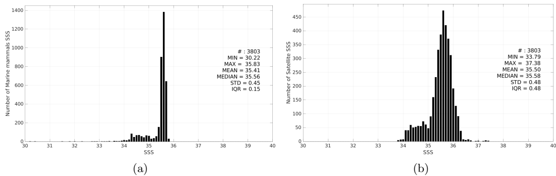
Figure 3: Histograms of SSS from Marine mammals (a) and SMOS SSS L4 v2 - Daily (BEC) (b) considering all match-up pairs per bins of 0.1 over the South Pacific Ocean Pi-MEP region and for the full satellite product period.
