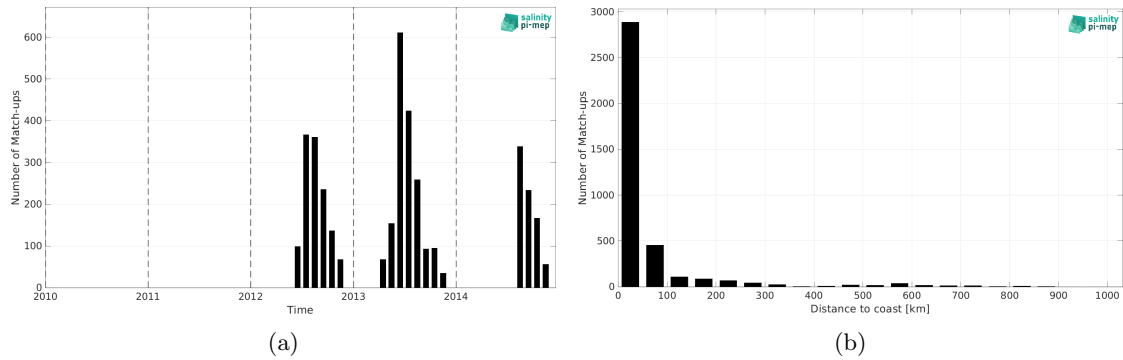
Figure 2: Number of match-ups between Marine mammals and SMOS SSS L4 v2 - Daily (BEC) SSS as a function of time (a) and as function of the distance to coast (b) over the South Pacific Ocean Pi-MEP region and for the full satellite product period.
