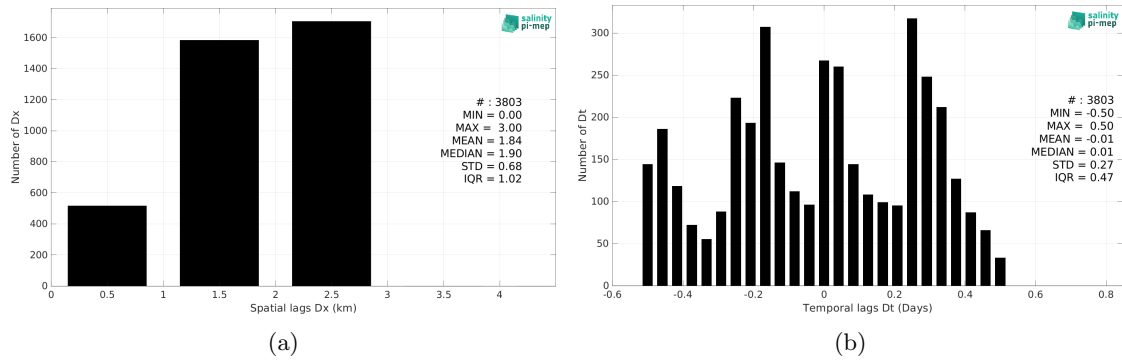
Figure 6: Histograms of the spatial (a) and temporal (b) lags between the location/time of the Marine mammals measurement and the date of the corresponding SMOS SSS L4 v2 - Daily (BEC) SSS pixel.
