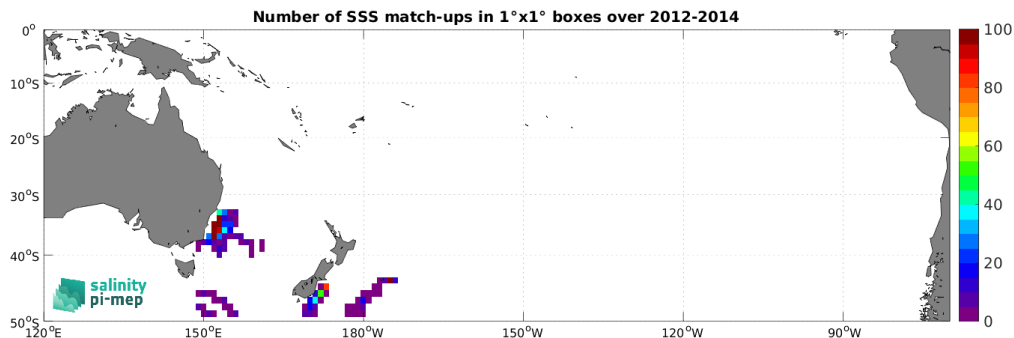
Figure 5: Number of SSS match-ups between Marine mammals SSS and the SMOS SSS L4 v2 - Daily (BEC) SSS product for the South Pacific Ocean Pi-MEP region over 1^\circ \times 1^\circ boxes and for the full satellite product period.
