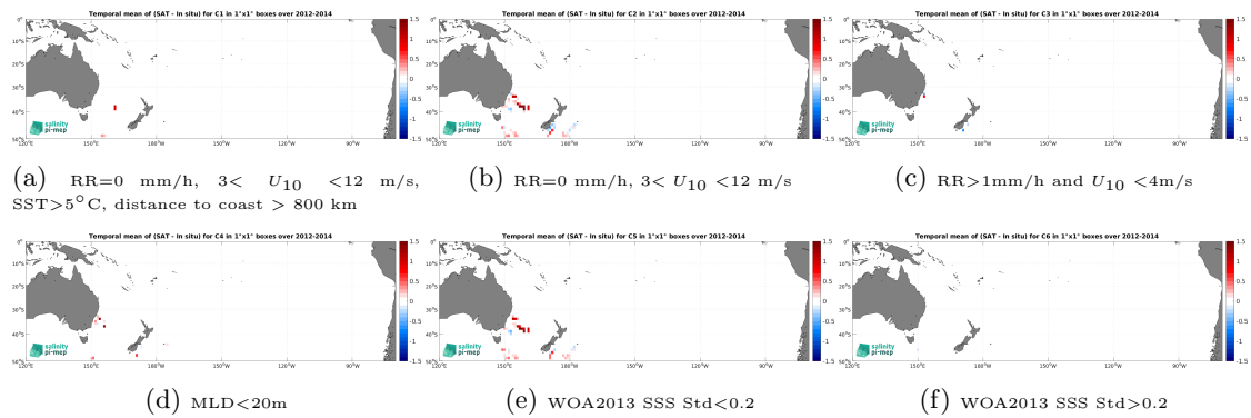
Figure 14: Temporal mean gridded over spatial boxes of size 1^\circ \times 1^\circ of \Delta SSS (SMOS SSS L4 v2 - Daily (BEC) - Marine mammals) for 6 different subdatasets corresponding to:RR=0 mm/h, 3 < U_{10} < 12 m/s, SST >5^\circ C, distance to coast > 800 km (a), RR=0 mm/h, 3 < U_{10} < 12 m/s (b), RR >1 mm/h and U_{10} < 4 m/s (c),MLD <20 m (d),WOA2013 SSS Std <0.2 (e),WOA2013 SSS Std >0.2 (f).
