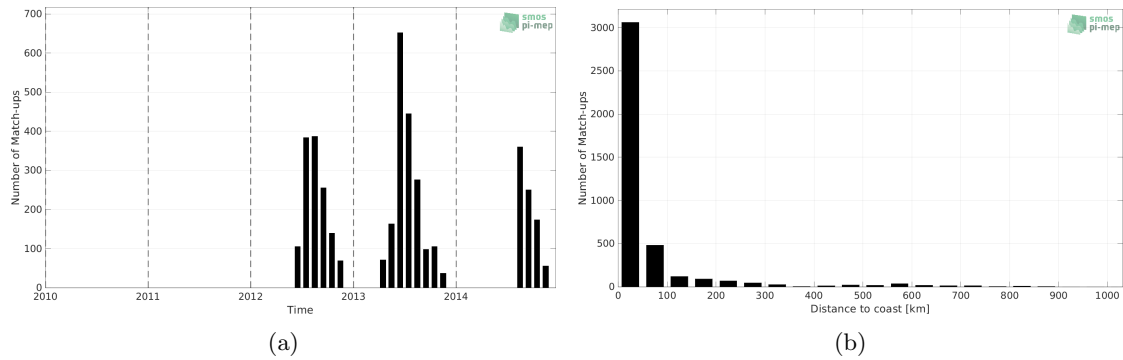
Figure 1: Number of match-ups between Marine mammals and SMOS SSS L4 v2 - Daily (BEC) SSS as a function of time (a) and as function of the distance to coast (b) over the South Pacific Ocean Pi-MEP region and for the full satellite product period.
