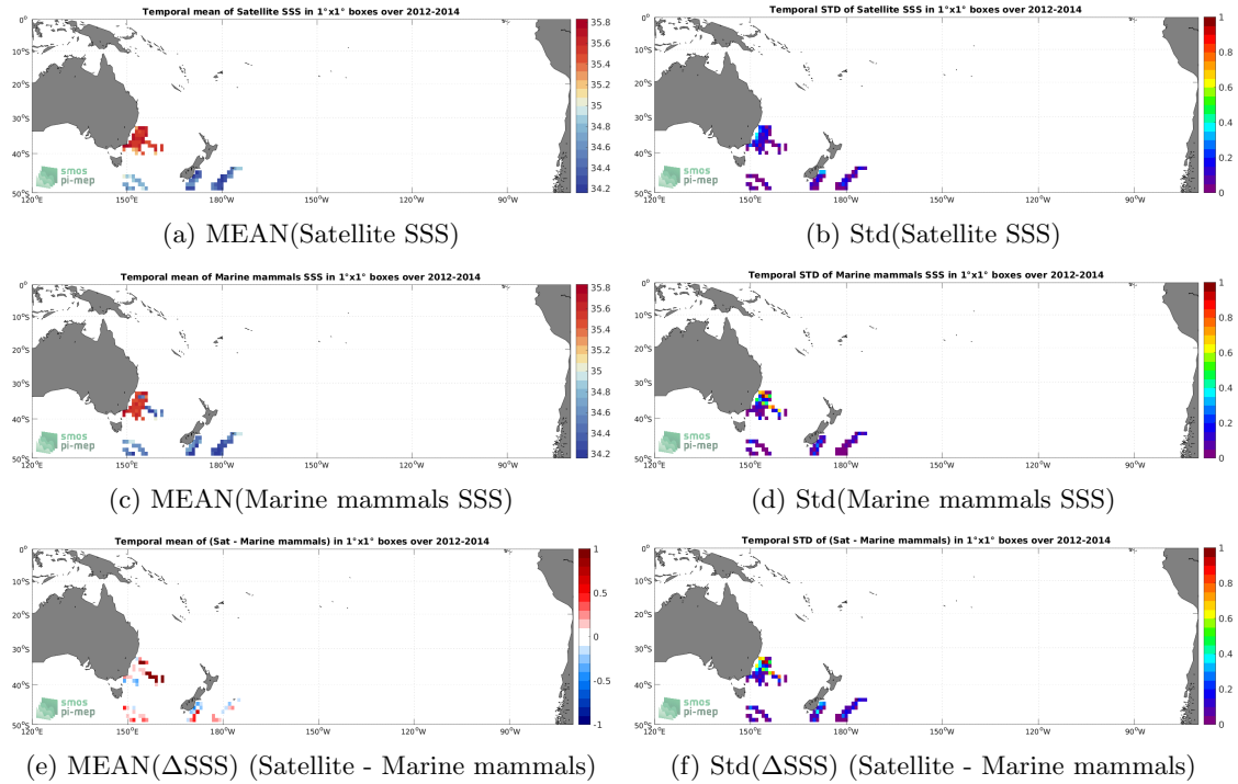
Figure 6: Temporal mean (left) and Std (right) of SSS from SMOS SSS L4 v2 - Daily (BEC) (top), Marine mammals (middle), and of \Delta SSS (Satellite - Marine mammals). Only match-up pairs are used to generate these maps.
