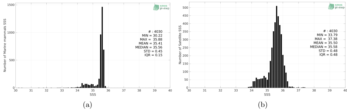
Figure 2: Histograms of SSS from Marine mammals (a) and SMOS SSS L4 v2 - Daily (BEC) (b) considering all match-up pairs per bins of 0.1 over the South Pacific Ocean Pi-MEP region and for the full satellite product period.
