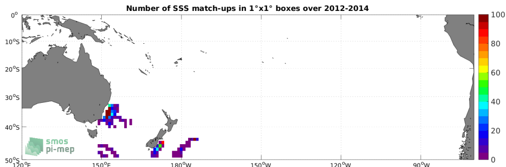
Figure 4: Number of SSS match-ups between Marine mammals SSS and the SMOS SSS L4 v2 - Daily (BEC) SSS product for the South Pacific Ocean Pi-MEP region over 1^\circ \times 1^\circ boxes and for the full satellite product period.
