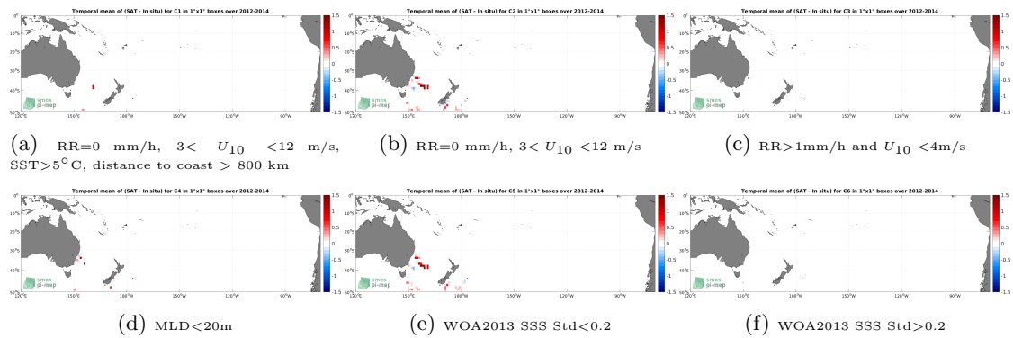
Figure 12: Temporal mean gridded over spatial boxes of size 1^\circ \times 1^\circ of \Delta SSS (SMOS SSS L4 v2 - Daily (BEC) - Marine mammals) for 6 different subdatasets corresponding to:RR=0 mm/h, 3 < U_{10} < 12 m/s, SST >5^\circ C, distance to coast > 800 km (a), RR=0 mm/h, 3 < U_{10} < 12 m/s (b), RR >1 mm/h and U_{10} < 4 m/s (c),MLD <20 m (d),WOA2013 SSS Std <0.2 (e),WOA2013 SSS Std >0.2 (f).
