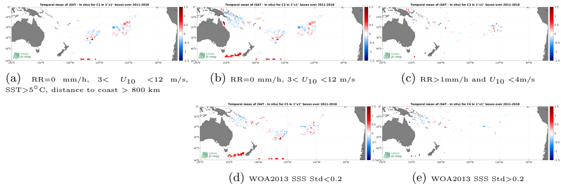
Figure 11: Temporal mean gridded over spatial boxes of size 1^\circ \times 1^\circ of \Delta SSS (SMOS SSS L4 v2 - Daily (BEC) - Surface drifters) for 5 different subdatasets corresponding to:RR=0 mm/h, 3 < U_{10} < 12 m/s, SST >5^\circ C, distance to coast > 800 km (a), RR=0 mm/h, 3 < U_{10} < 12 m/s (b), RR >1 mm/h and U_{10} < 4 m/s (c), WOA2013 SSS Std <0.2 (d), WOA2013 SSS Std >0.2 (e).
