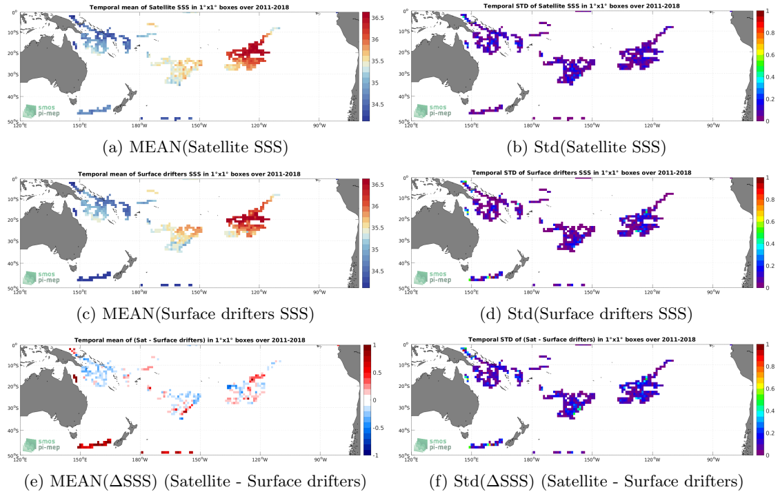
Figure 5: Temporal mean (left) and Std (right) of SSS from SMOS SSS L4 v2 - Daily (BEC) (top), Surface drifters (middle), and of \Delta SSS (Satellite - Surface drifters). Only match-up pairs are used to generate these maps.
