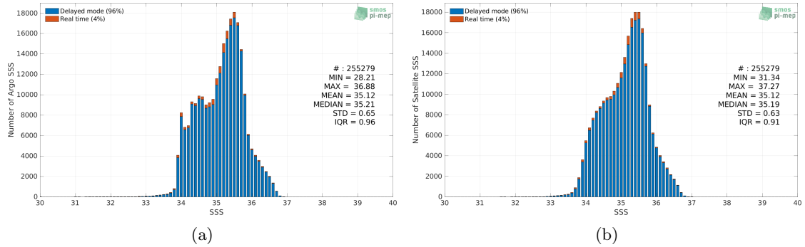
Figure 2: Histograms of SSS from Argo (a) and SMOS SSS L4 v2 - Daily (BEC) (b) considering all match-up pairs per bins of 0.1 over the South Pacific Ocean Pi-MEP region and for the full satellite product period.
