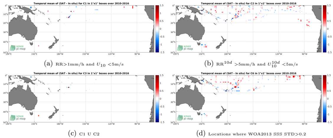
Figure 12: Temporal mean gridded over spatial boxes of size 1^\circ \times 1^\circ of \Delta SSS (SMOS-L3-ICDC-V3-MONTHLY-0.5DEG - TSG-SAMOS) for 4 different subdatasets corresponding to: RR > 1\text{mm/h} and U_{10} < 5\text{m/s} (a), RR^{10d} > 5\text{mm/h} and U_{10}^{10d} < 5\text{m/s} (b), C1 U C2 (c), Locations where WOA2013 SSS STD > 0.2 (d).
