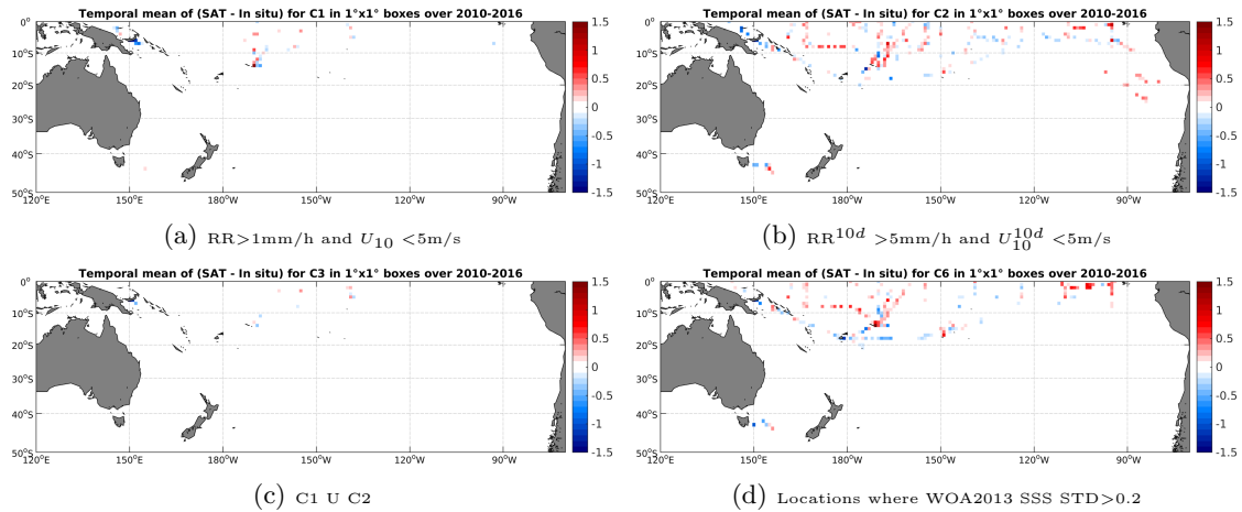
Figure 12: Temporal mean gridded over spatial boxes of size 1^\circ \times 1^\circ of \Delta SSS (SMOS-L3-ICDC-V3-MONTHLY-0.5DEG - TSG-SAMOS) for 4 different subdatasets corresponding to:RR > 1 mm/h and U_{10} < 5 m/s (a), RR^{10d} > 5 mm/h and U_{10}^{10d} < 5 m/s (b), C1 U C2 (c),Locations where WOA2013 SSS STD > 0.2 (d).
