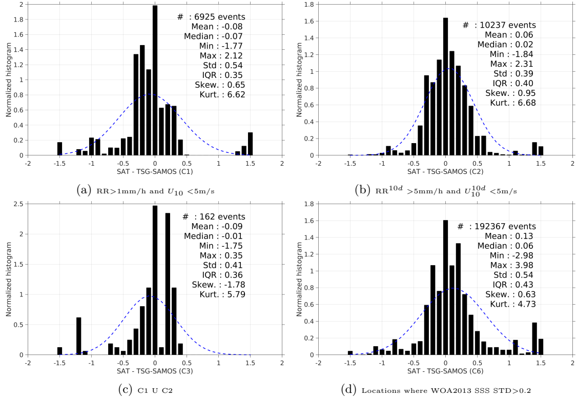
Figure 13: Normalized histogram of \Delta\text{SSS} (SMOS-L3-ICDC-V3-MONTHLY-0.5DEG - TSG-SAMOS) for 6 different subdatasets corresponding to: RR > 1mm/h and U_{10} < 5\text{m/s} (a), \text{RR}^{10d} > 5\text{mm/h} and U_{10}^{10d} < 5\text{m/s} (b), C1 U C2 (c), Locations where WOA2013 SSS STD > 0.2 (d).
