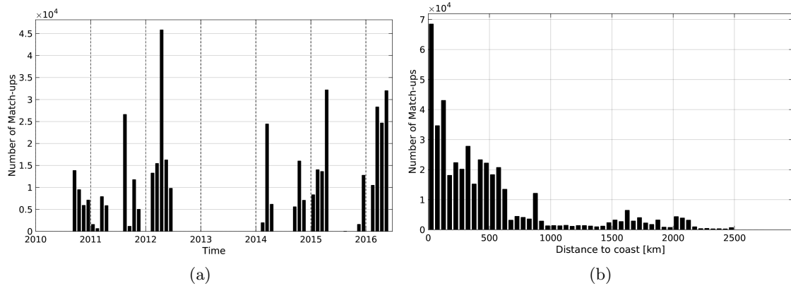
Figure 1: Number of match-ups between TSG-SAMOS and SMOS-L3-ICDC-V3-MONTHLY-0.5DEG SSS as a function of time (a) and as function of the distance to coast (b) over the South Pacific Ocean Pi-MEP region and for the full satellite product period.
