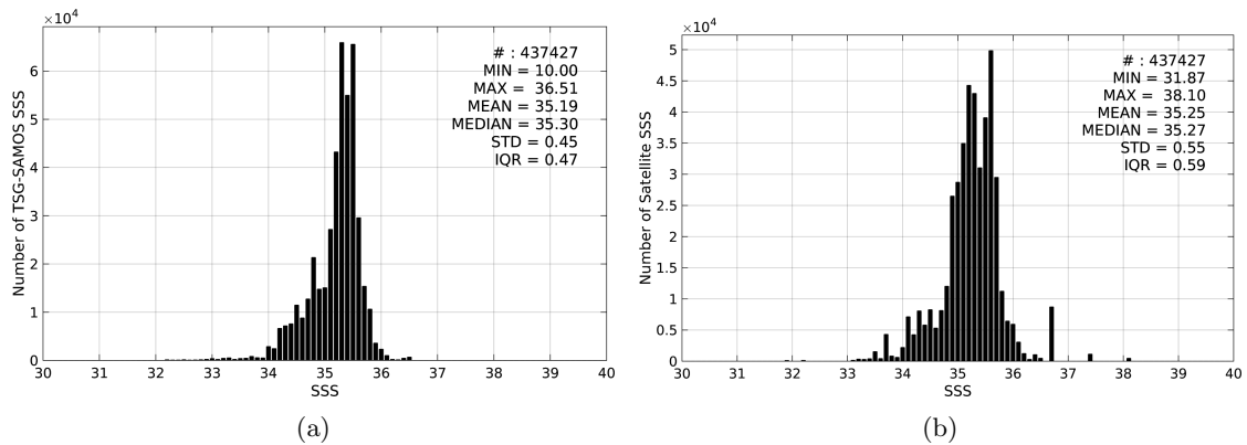
Figure 2: Histograms of SSS from TSG-SAMOS (a) and SMOS-L3-ICDC-V3-MONTHLY-0.5DEG (b) considering all match-up pairs per bins of 0.1 over the South Pacific Ocean Pi-MEP region and for the full satellite product period.
