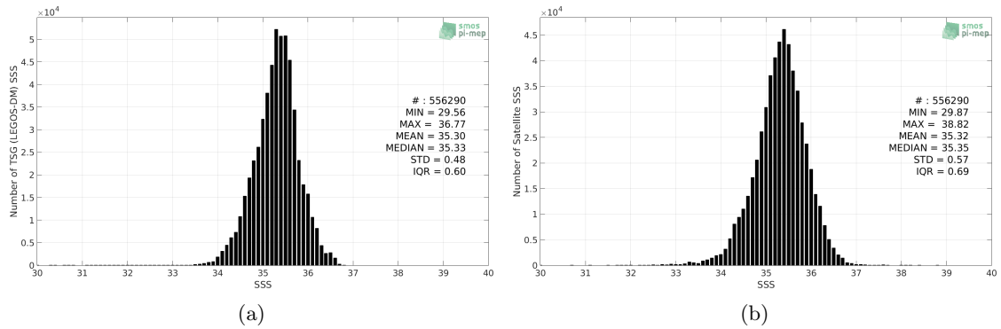
Figure 2: Histograms of SSS from TSG (LEGOS-DM) (a) and SMOS SSS L3 v3 Monthly (ICDC) (b) considering all match-up pairs per bins of 0.1 over the South Pacific Ocean Pi-MEP region and for the full satellite product period.
