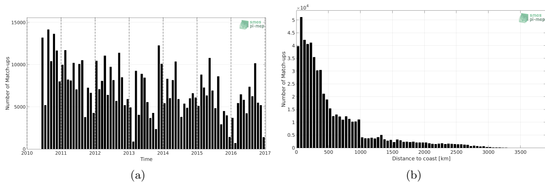
Figure 1: Number of match-ups between TSG (LEGOS-DM) and SMOS SSS L3 v3 Monthly (ICDC) SSS as a function of time (a) and as function of the distance to coast (b) over the South Pacific Ocean Pi-MEP region and for the full satellite product period.
