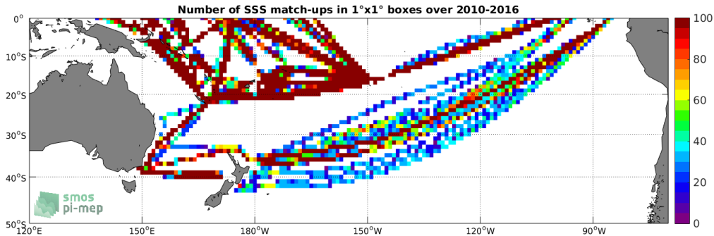
Figure 4: Number of SSS match-ups between TSG (LEGOS-DM) SSS and the SMOS SSS L3 v3 Monthly (ICDC) SSS product for the South Pacific Ocean Pi-MEP region over 1^\circ \times 1^\circ boxes and for the full satellite product period.
