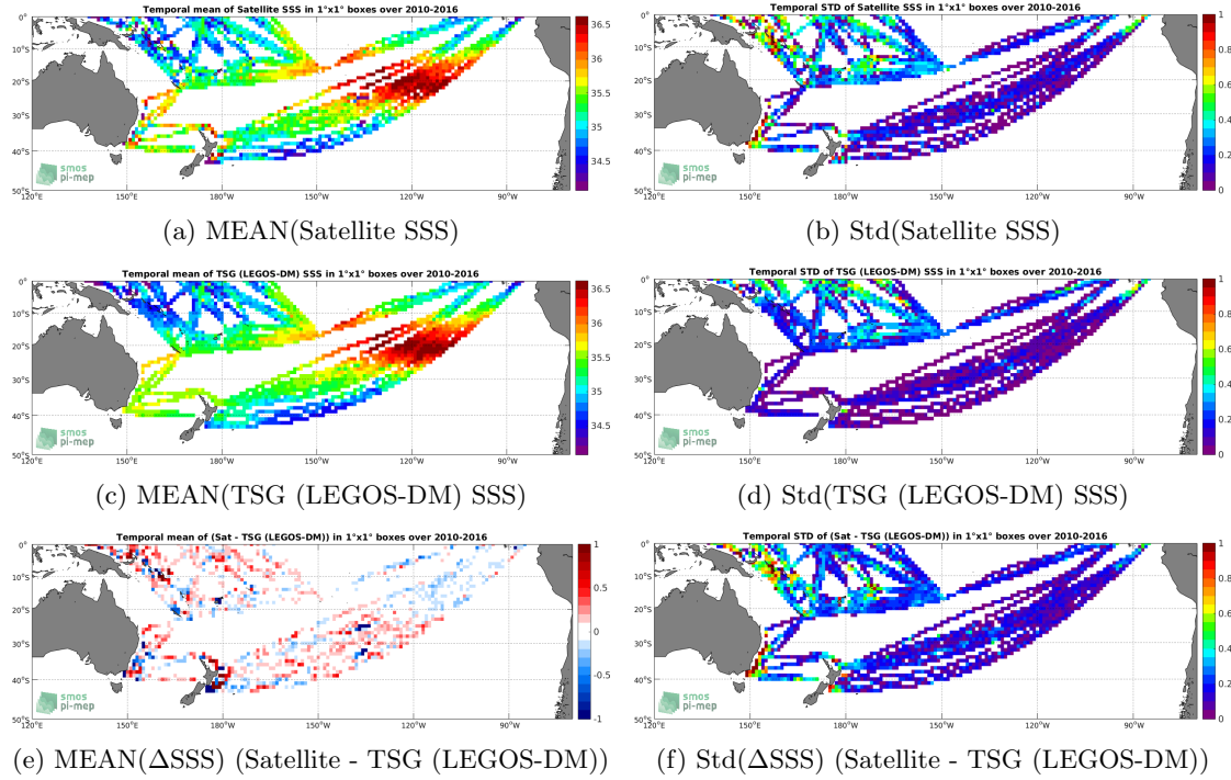
Figure 6: Temporal mean (left) and Std (right) of SSS from SMOS SSS L3 v3 Monthly (ICDC) (top), TSG (LEGOS-DM) (middle), and of \Delta SSS (Satellite - TSG (LEGOS-DM)). Only match-up pairs are used to generate these maps.
