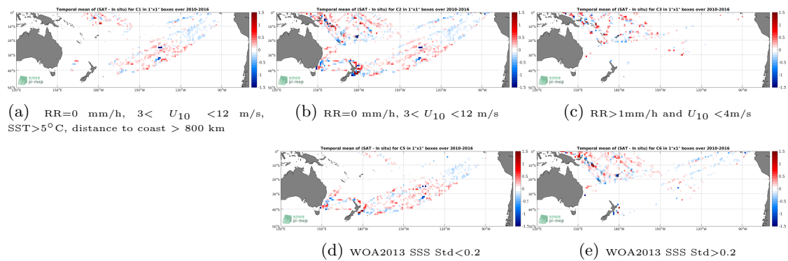
Figure 12: Temporal mean gridded over spatial boxes of size 1^\circ \times 1^\circ of \Delta\text{SSS} (SMOS SSS L3 v3 Monthly (ICDC) - TSG (LEGOS-DM)) for 5 different subdatasets corresponding to:RR=0 mm/h, 3 < U_{10} < 12 m/s, SST >5^\circ\text{C} , distance to coast > 800 km (a), RR=0 mm/h, 3 < U_{10} < 12 m/s (b), RR >1 mm/h and U_{10} < 4 m/s (c), WOA2013 SSS Std <0.2 (d), WOA2013 SSS Std >0.2 (e).
