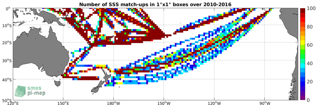
Figure 4: Number of SSS match-ups between TSG (LEGOS-DM) SSS and the SMOS SSS L3 v3 Monthly (ICDC) SSS product for the South Pacific Ocean Pi-MEP region over 1°x1° boxes and for the full satellite product period.
