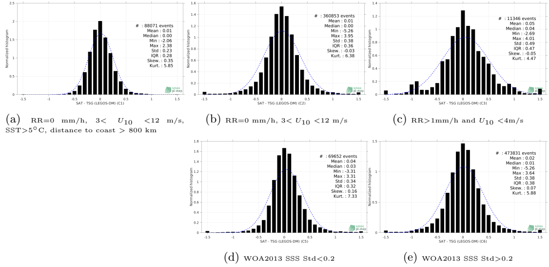
Figure 13: Normalized histogram of \Delta\text{SSS} (SMOS SSS L3 v3 Monthly (ICDC) - TSG (LEGOS-DM)) for 5 different subdatasets corresponding to: RR=0 mm/h, 3 < U_{10} < 12 m/s, SST>5°C, distance to coast > 800 km (a), RR=0 mm/h, 3 < U_{10} < 12 m/s (b), RR>1mm/h and U_{10} < 4 m/s (c), WOA2013 SSS Std<0.2 (d), WOA2013 SSS Std>0.2 (e).
