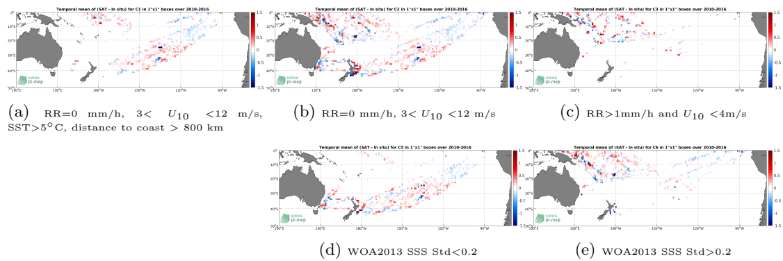
Figure 12: Temporal mean gridded over spatial boxes of size 1^\circ \times 1^\circ of \Delta SSS (SMOS SSS L3 v3 Monthly (ICDC) - TSG (LEGOS-DM)) for 5 different subdatasets corresponding to:RR=0 mm/h, 3 < U_{10} < 12 m/s, SST >5^\circ C, distance to coast > 800 km (a), RR=0 mm/h, 3 < U_{10} < 12 m/s (b), RR >1 mm/h and U_{10} < 4 m/s (c), WOA2013 SSS Std <0.2 (d), WOA2013 SSS Std >0.2 (e).
