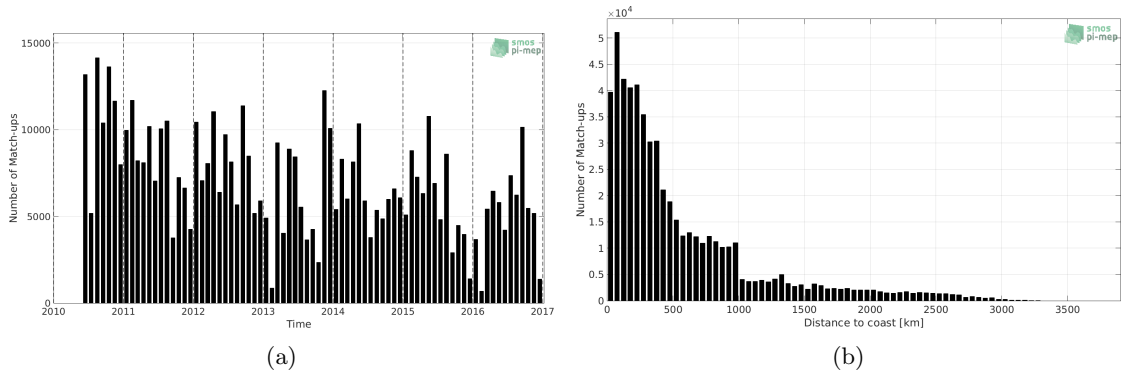
Figure 1: Number of match-ups between TSG-LEGOS-DM and SMOS-L3-ICDC-V3-MONTHLY-0.5DEG SSS as a function of time (a) and as function of the distance to coast (b) over the South Pacific Ocean Pi-MEP region and for the full satellite product period.
