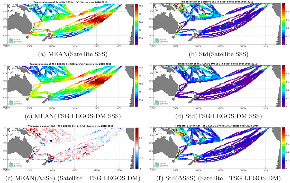
Figure 6: Temporal mean (left) and Std (right) of SSS from SMOS-L3-ICDC-V3-MONTHLY-0.5DEG (top), TSG-LEGOS-DM (middle), and of \Delta SSS (Satellite - TSG-LEGOS-DM). Only match-up pairs are used to generate these maps.
