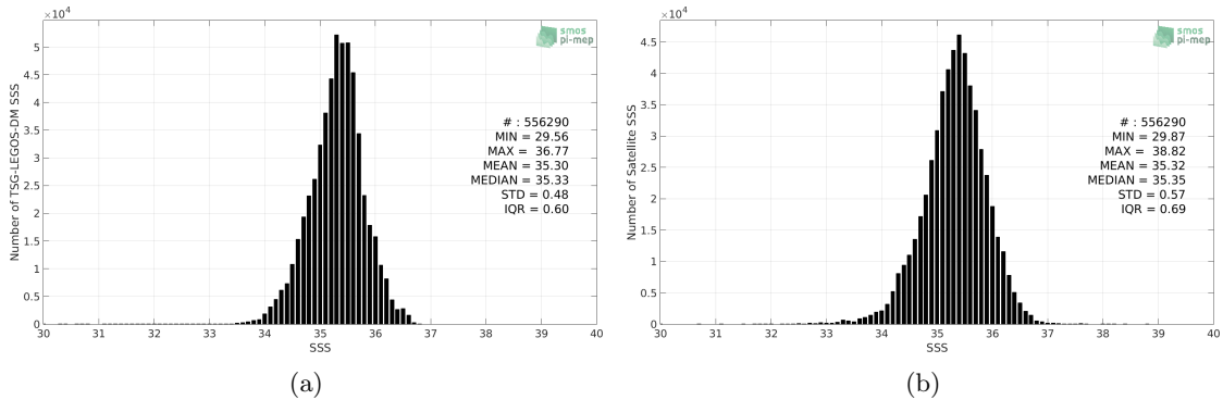
Figure 2: Histograms of SSS from TSG-LEGOS-DM (a) and SMOS-L3-ICDC-V3-MONTHLY-0.5DEG (b) considering all match-up pairs per bins of 0.1 over the South Pacific Ocean Pi-MEP region and for the full satellite product period.
