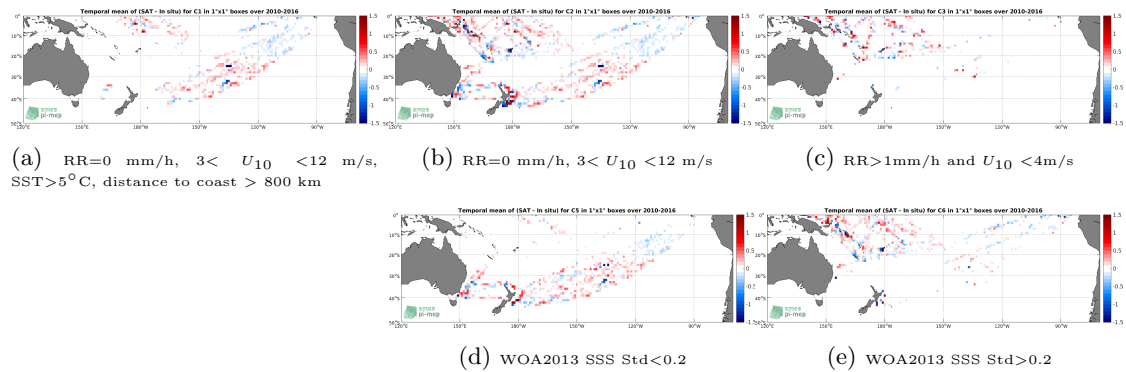
Figure 12: Temporal mean gridded over spatial boxes of size 1^\circ \times 1^\circ of \Delta SSS (SMOS-L3-ICDC-V3-MONTHLY-0.5DEG - TSG-LEGOS-DM) for 5 different subdatasets corresponding to:RR=0 mm/h, 3 < U_{10} < 12 m/s, SST > 5^\circ\text{C} , distance to coast > 800 km (a), RR=0 mm/h, 3 < U_{10} < 12 m/s (b), RR > 1 mm/h and U_{10} < 4 m/s (c), WOA2013 SSS Std < 0.2 (d), WOA2013 SSS Std > 0.2 (e).
