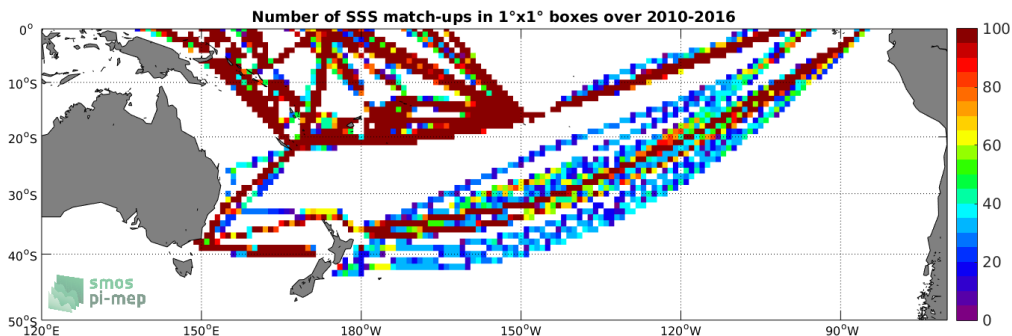
Figure 4: Number of SSS match-ups between TSG-LEGOS-DM SSS and the SMOS-L3-ICDC-V3-MONTHLY-0.5DEG SSS product for the South Pacific Ocean Pi-MEP region over 1^\circ \times 1^\circ boxes and for the full satellite product period.
