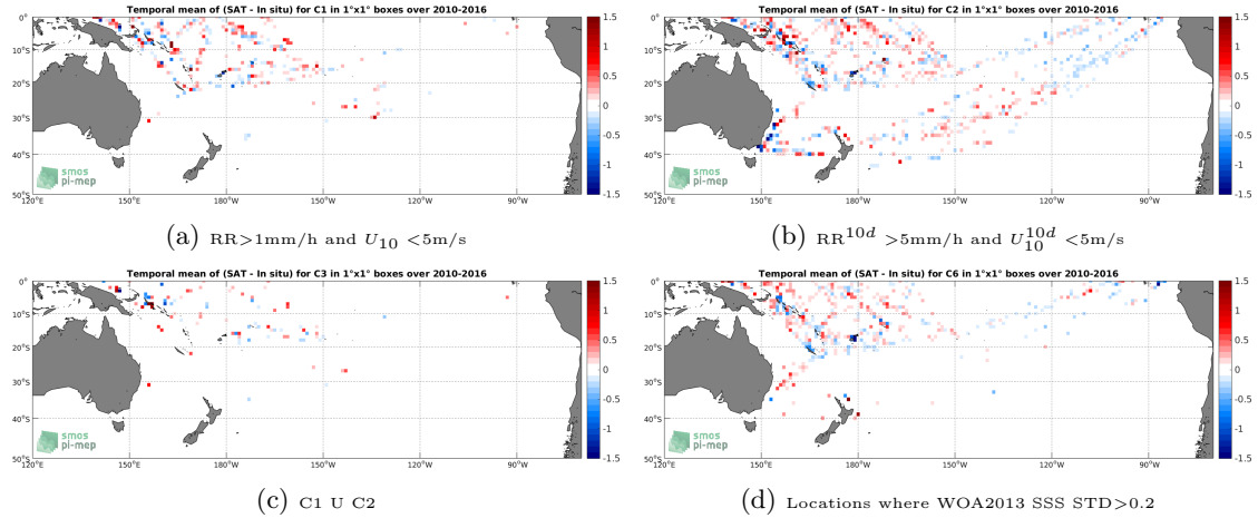
Figure 12: Temporal mean gridded over spatial boxes of size 1^\circ \times 1^\circ of \Delta SSS (SMOS-L3-ICDC-V3-MONTHLY-0.5DEG - TSG-LEGOS-DM) for 4 different subdatasets corresponding to: RR > 1\text{mm/h} and U_{10} < 5\text{m/s} (a), RR^{10d} > 5\text{mm/h} and U_{10}^{10d} < 5\text{m/s} (b), C1 \cup C2 (c), Locations where WOA2013 SSS STD > 0.2 (d).
