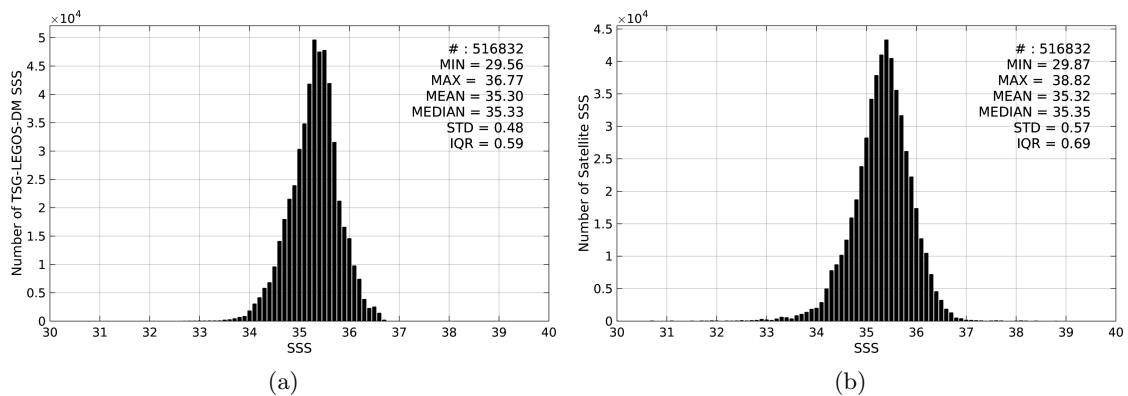
Figure 2: Histograms of SSS from TSG-LEGOS-DM (a) and SMOS-L3-ICDC-V3-MONTHLY-0.5DEG (b) considering all match-up pairs per bins of 0.1 over the South Pacific Ocean Pi-MEP region and for the full satellite product period.
