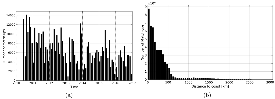
Figure 1: Number of match-ups between TSG-LEGOS-DM and SMOS-L3-ICDC-V3-MONTHLY-0.5DEG SSS as a function of time (a) and as function of the distance to coast (b) over the South Pacific Ocean Pi-MEP region and for the full satellite product period.
