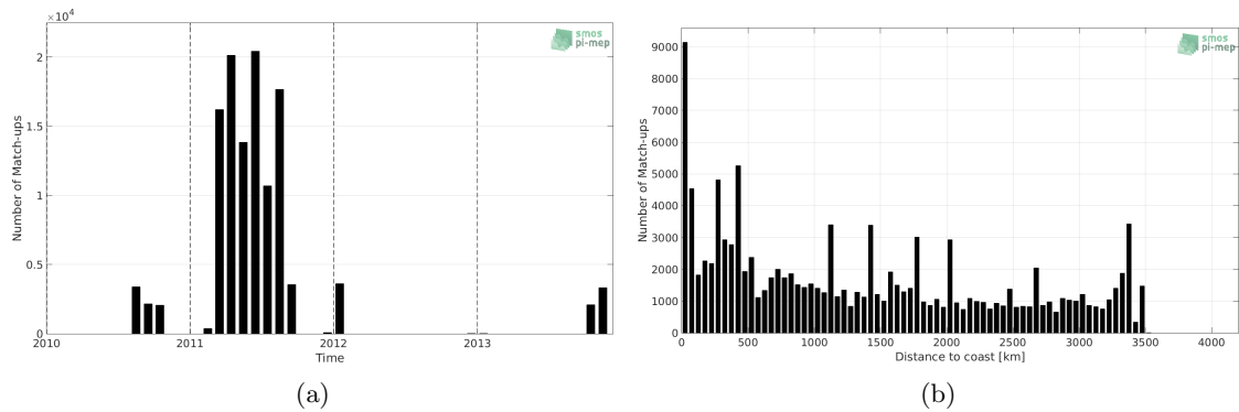
Figure 1: Number of match-ups between TSG (GOSUD-Sailing-ship) and SMOS SSS L3 v3 Monthly (ICDC) SSS as a function of time (a) and as function of the distance to coast (b) over the South Pacific Ocean Pi-MEP region and for the full satellite product period.
