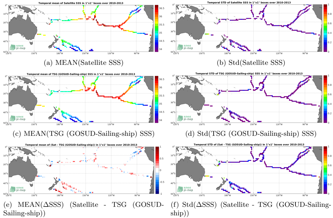
Figure 6: Temporal mean (left) and Std (right) of SSS from SMOS SSS L3 v3 Monthly (ICDC) (top), TSG (GOSUD-Sailing-ship) (middle), and of \Delta SSS (Satellite - TSG (GOSUD-Sailing-ship)). Only match-up pairs are used to generate these maps.
