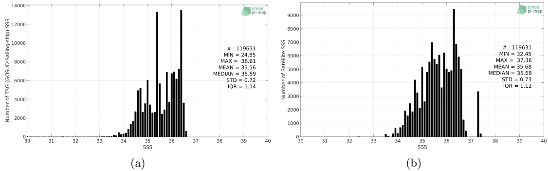
Figure 2: Histograms of SSS from TSG (GOSUD-Sailing-ship) (a) and SMOS SSS L3 v3 Monthly (ICDC) (b) considering all match-up pairs per bins of 0.1 over the South Pacific Ocean Pi-MEP region and for the full satellite product period.
