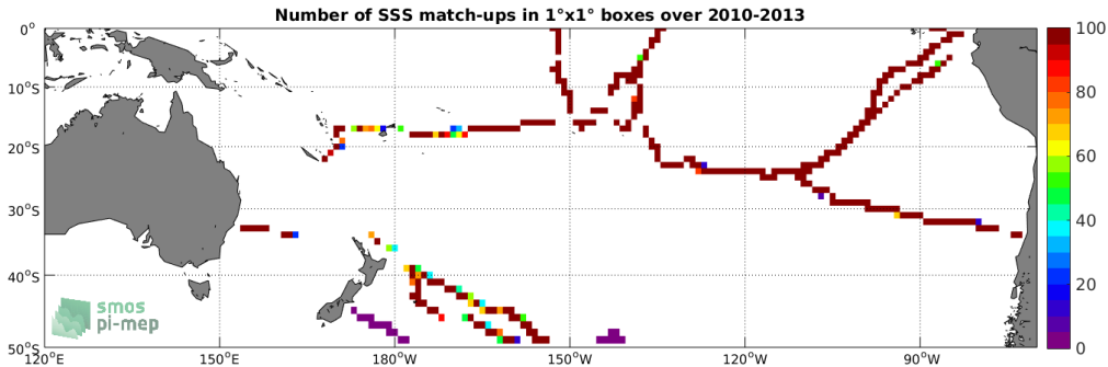
Figure 4: Number of SSS match-ups between TSG (GOSUD-Sailing-ship) SSS and the SMOS SSS L3 v3 Monthly (ICDC) SSS product for the South Pacific Ocean Pi-MEP region over 1^\circ \times 1^\circ boxes and for the full satellite product period.
