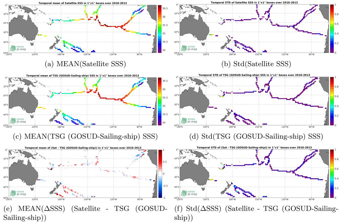
Figure 6: Temporal mean (left) and Std (right) of SSS from SMOS SSS L3 v3 Monthly (ICDC) (top), TSG (GOSUD-Sailing-ship) (middle), and of \Delta SSS (Satellite - TSG (GOSUD-Sailing-ship)). Only match-up pairs are used to generate these maps.
