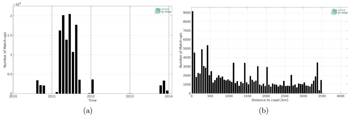
Figure 1: Number of match-ups between TSG-GOSUD-Sailing-ship and SMOS-L3-ICDC-V3-MONTHLY-0.5DEG SSS as a function of time (a) and as function of the distance to coast (b) over the South Pacific Ocean Pi-MEP region and for the full satellite product period.
