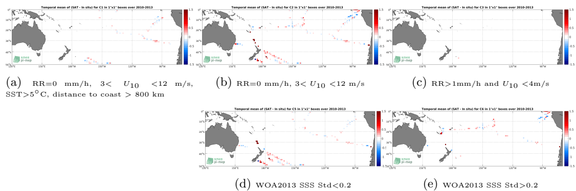
Figure 12: Temporal mean gridded over spatial boxes of size 1^\circ \times 1^\circ of \Delta SSS (SMOS-L3-ICDC-V3-MONTHLY-0.5DEG - TSG-GOSUD-Sailing-ship) for 5 different subdatasets corresponding to:RR=0 mm/h, 3 < U_{10} < 12 m/s, SST >5^\circ\text{C} , distance to coast > 800 km (a), RR=0 mm/h, 3 < U_{10} < 12 m/s (b), RR >1 mm/h and U_{10} < 4 m/s (c), WOA2013 SSS Std <0.2 (d), WOA2013 SSS Std >0.2 (e).
