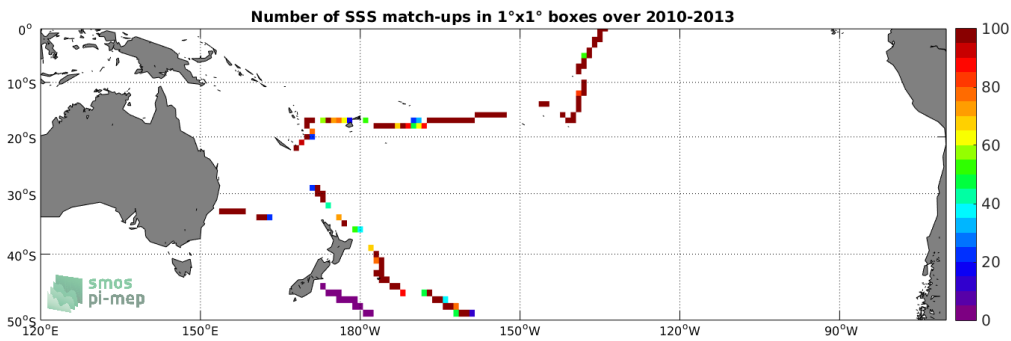
Figure 4: Number of SSS match-ups between TSG-GOSUD-Sailing-ship SSS and the SMOS-L3-ICDC-V3-MONTHLY-0.5DEG SSS product for the South Pacific Ocean Pi-MEP region over 1^\circ \times 1^\circ boxes and for the full satellite product period.
