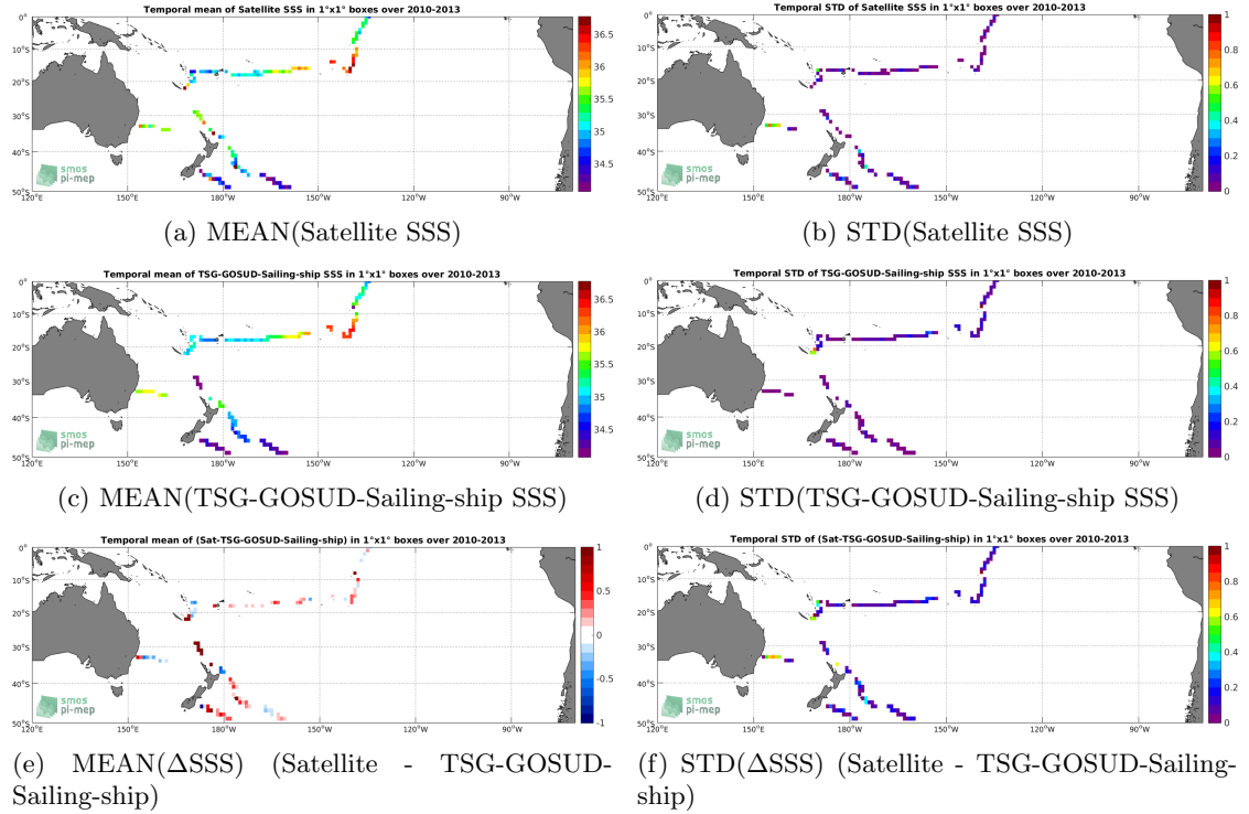
Figure 6: Temporal mean (left) and STD (right) of SSS from SMOS-L3-ICDC-V3-MONTHLY-0.5DEG (top), TSG-GOSUD-Sailing-ship (middle), and of \Delta SSS (Satellite - TSG-GOSUD-Sailing-ship). Only match-up pairs are used to generate these maps.
