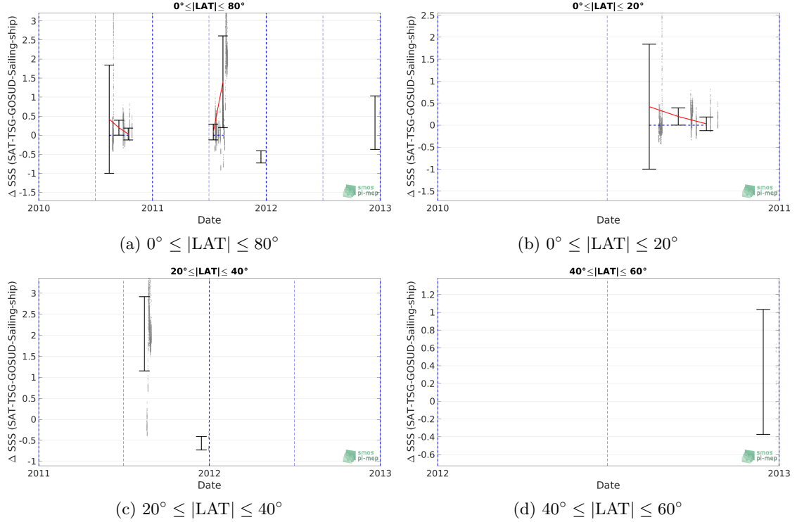
Figure 10: Monthly-averaged mean (red curves) \Delta SSS (Satellite - TSG-GOSUD-Sailing-ship) and \pm 1 STD (black vertical thick bars) as function of time for all the collected Pi-MEP match-up pairs estimated over the South Pacific Ocean Pi-MEP region and for the full satellite product period are shown for different latitude bands: (a) Latitude band 80^\circ\text{S}-80^\circ\text{N} , (b) latitude band 20^\circ\text{S}-20^\circ\text{N} , (c) Mid Latitude bands 40^\circ\text{S}-20^\circ\text{S} and 20^\circ\text{N}-40^\circ\text{N} and (d) Latitude bands 60^\circ\text{S}-40^\circ\text{S} and 40^\circ\text{N}-60^\circ\text{N} .
