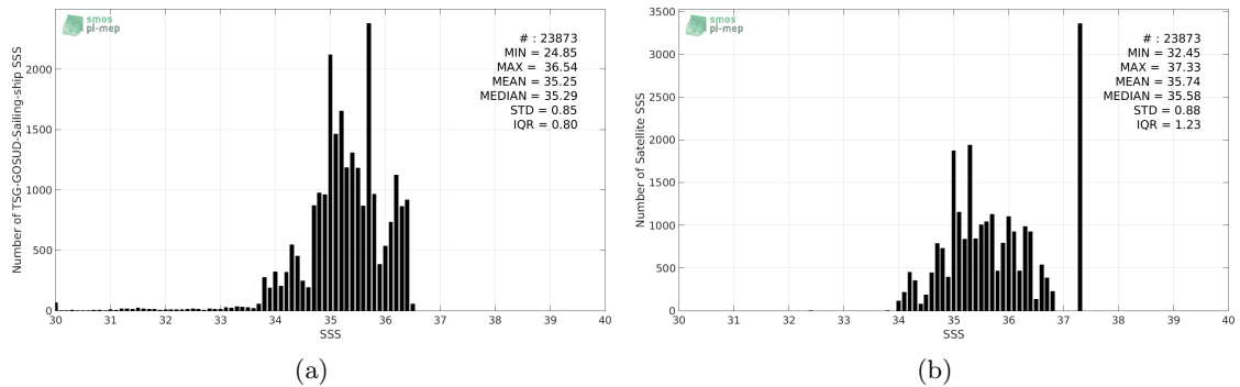
Figure 2: Histograms of SSS from TSG-GOSUD-Sailing-ship (a) and SMOS-L3-ICDC-V3-MONTHLY-0.5DEG (b) considering all match-up pairs per bins of 0.1 over the South Pacific Ocean Pi-MEP region and for the full satellite product period.
