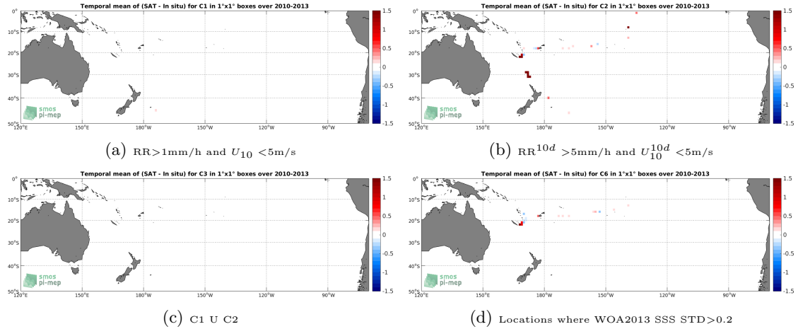
Figure 12: Temporal mean gridded over spatial boxes of size 1^\circ \times 1^\circ of \Delta SSS (SMOS-L3-ICDC-V3-MONTHLY-0.5DEG - TSG-GOSUD-Sailing-ship) for 4 different subdatasets corresponding to: RR > 1\text{mm/h} and U_{10} < 5\text{m/s} (a), RR^{10d} > 5\text{mm/h} and U_{10}^{10d} < 5\text{m/s} (b), C1 U C2 (c), Locations where WOA2013 SSS STD > 0.2 (d).
