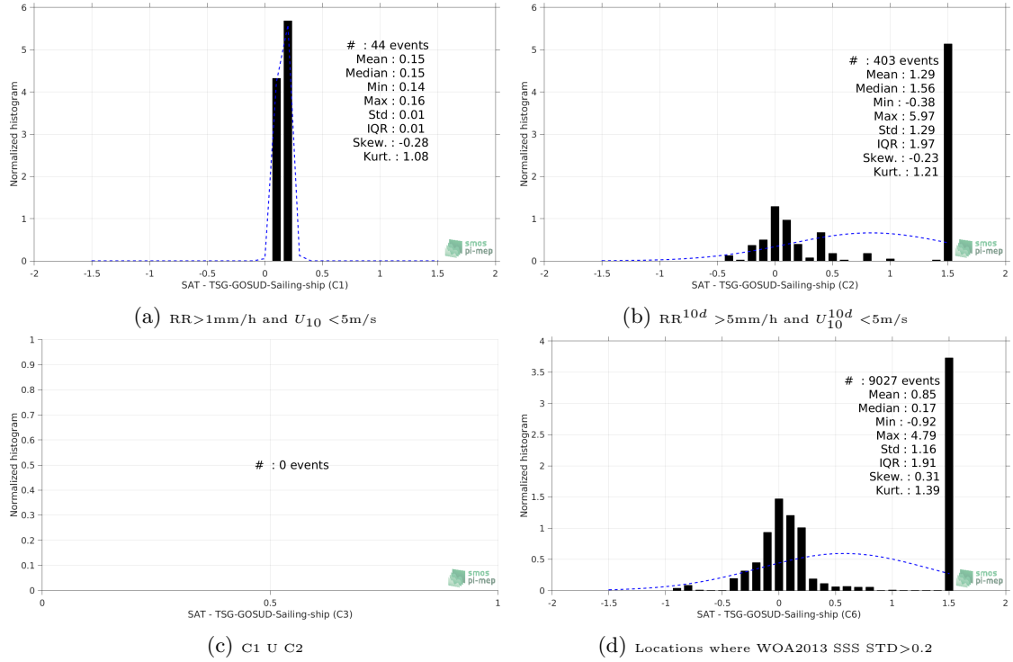
Figure 13: Normalized histogram of \Delta\text{SSS} (SMOS-L3-ICDC-V3-MONTHLY-0.5DEG - TSG-GOSUD-Sailing-ship) for 6 different subdatasets corresponding to: RR > 1\text{mm/h} and U_{10} < 5\text{m/s} (a), RR^{10d} > 5\text{mm/h} and U_{10}^{10d} < 5\text{m/s} (b), C1 U C2 (c), Locations where WOA2013 SSS STD > 0.2 (d).
