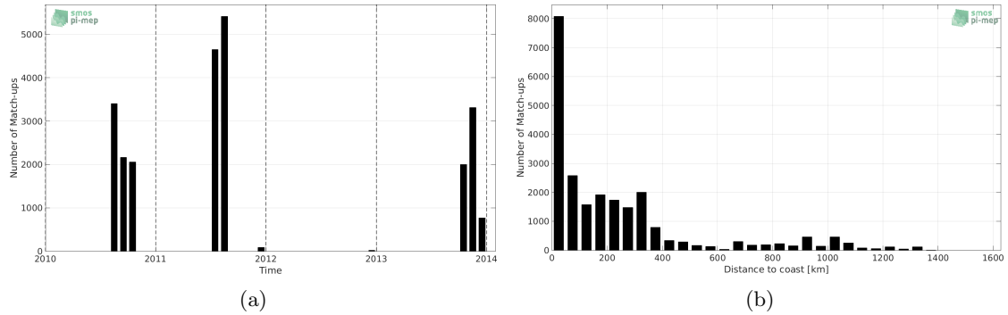
Figure 1: Number of match-ups between TSG-GOSUD-Sailing-ship and SMOS-L3-ICDC-V3-MONTHLY-0.5DEG SSS as a function of time (a) and as function of the distance to coast (b) over the South Pacific Ocean Pi-MEP region and for the full satellite product period.
