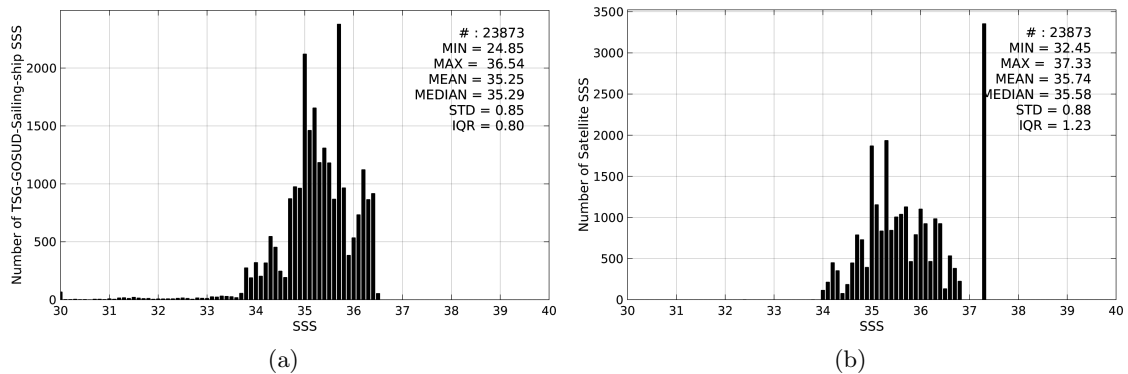
Figure 2: Histograms of SSS from TSG-GOSUD-Sailing-ship (a) and SMOS-L3-ICDC-V3-MONTHLY-0.5DEG (b) considering all match-up pairs per bins of 0.1 over the South Pacific Ocean Pi-MEP region and for the full satellite product period.
