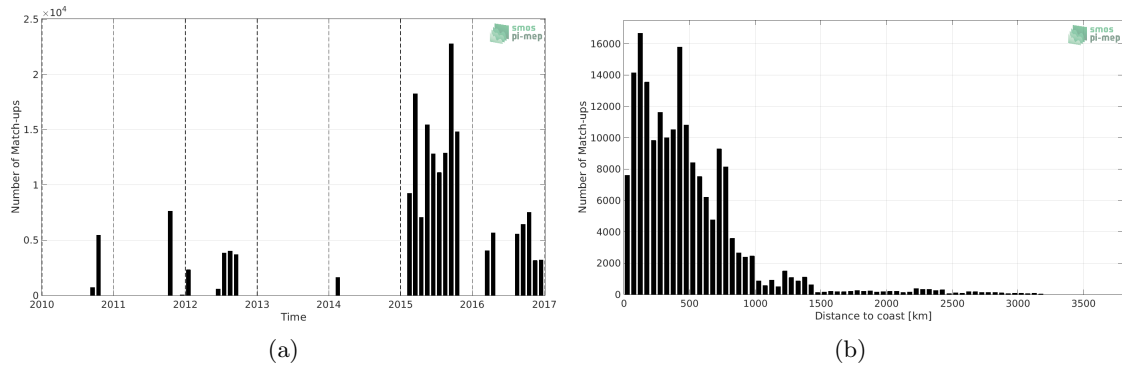
Figure 1: Number of match-ups between TSG (GOSUD-Research-vessel) and SMOS SSS L3 v3 Monthly (ICDC) SSS as a function of time (a) and as function of the distance to coast (b) over the South Pacific Ocean Pi-MEP region and for the full satellite product period.
