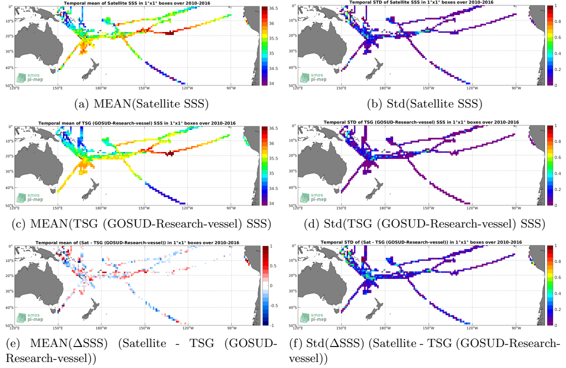
Figure 6: Temporal mean (left) and Std (right) of SSS from SMOS SSS L3 v3 Monthly (ICDC) (top), TSG (GOSUD-Research-vessel) (middle), and of \Delta SSS (Satellite - TSG (GOSUD-Research-vessel)). Only match-up pairs are used to generate these maps.
