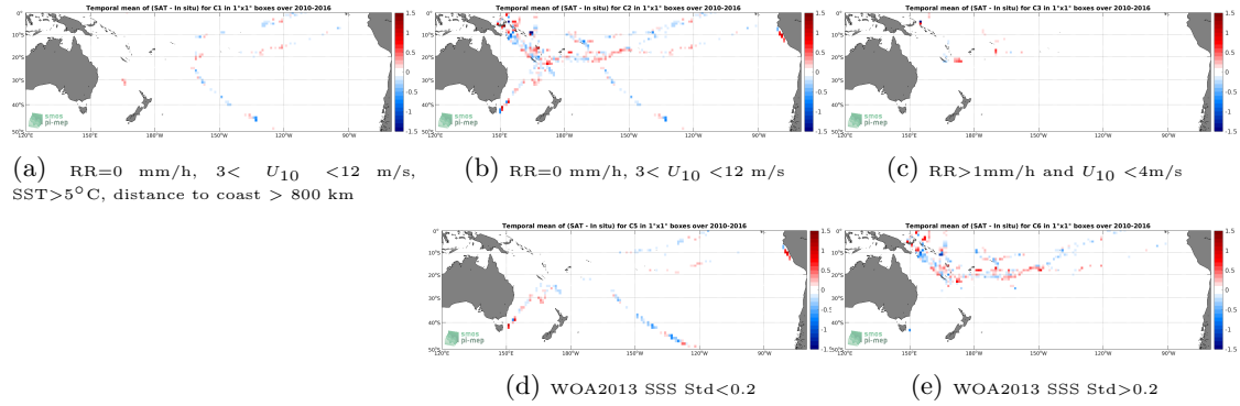
Figure 12: Temporal mean gridded over spatial boxes of size 1^\circ \times 1^\circ of \Delta SSS (SMOS SSS L3 v3 Monthly (ICDC) - TSG (GOSUD-Research-vessel)) for 5 different subdatasets corresponding to: RR=0 mm/h, 3 < U_{10} < 12 m/s, SST >5^\circ\text{C} , distance to coast > 800 km (a), RR=0 mm/h, 3 < U_{10} < 12 m/s (b), RR>1\text{mm/h} and U_{10} < 4\text{m/s} (c), WOA2013 SSS Std <0.2 (d), WOA2013 SSS Std >0.2 (e).
