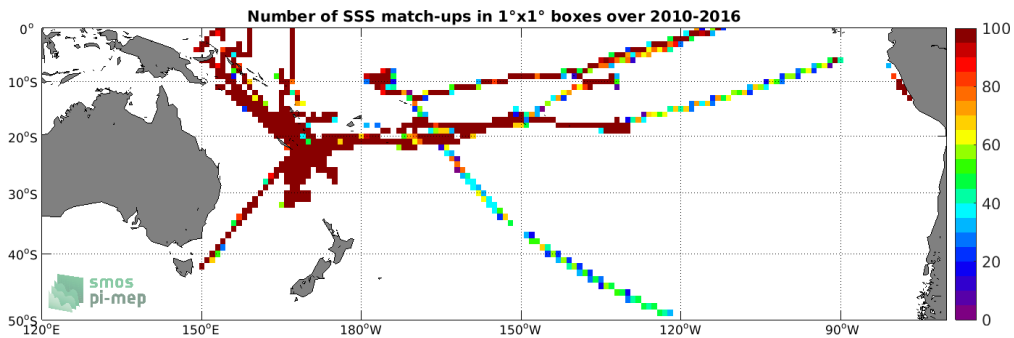
Figure 4: Number of SSS match-ups between TSG (GOSUD-Research-vessel) SSS and the SMOS SSS L3 v3 Monthly (ICDC) SSS product for the South Pacific Ocean Pi-MEP region over 1°x1° boxes and for the full satellite product period.
