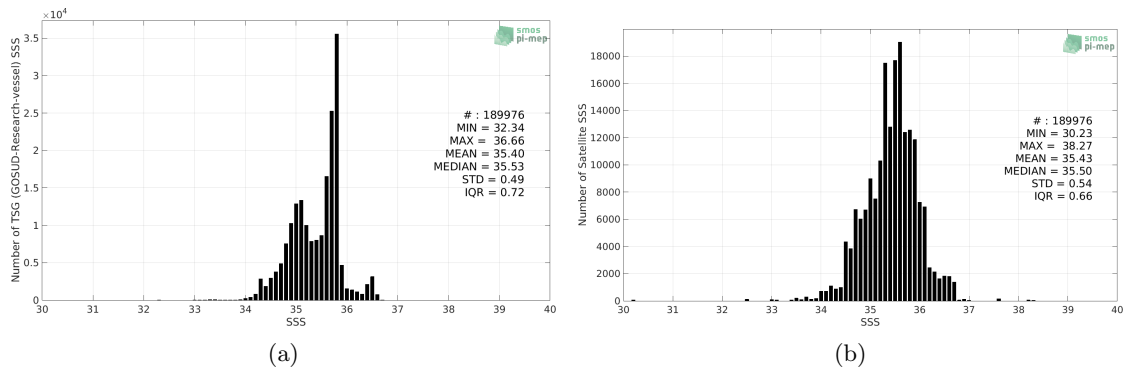
Figure 2: Histograms of SSS from TSG (GOSUD-Research-vessel) (a) and SMOS SSS L3 v3 Monthly (ICDC) (b) considering all match-up pairs per bins of 0.1 over the South Pacific Ocean Pi-MEP region and for the full satellite product period.
