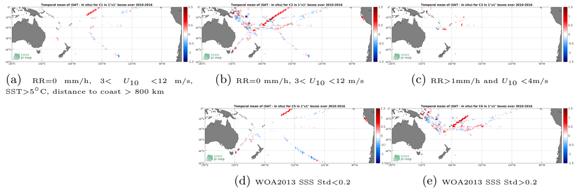
Figure 12: Temporal mean gridded over spatial boxes of size 1^\circ \times 1^\circ of \Delta SSS (SMOS-L3-ICDC-V3-MONTHLY-0.5DEG - TSG-GOSUD-Research-vessel) for 5 different subdatasets corresponding to: RR=0 mm/h, 3 < U_{10} < 12 m/s, SST > 5^\circ C , distance to coast > 800 km (a), RR=0 mm/h, 3 < U_{10} < 12 m/s (b), RR > 1 mm/h and U_{10} < 4 m/s (c), WOA2013 SSS Std < 0.2 (d), WOA2013 SSS Std > 0.2 (e).
