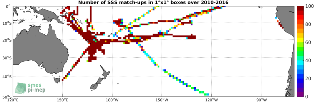
Figure 4: Number of SSS match-ups between TSG-GOSUD-Research-vessel SSS and the SMOS-L3-ICDC-V3-MONTHLY-0.5DEG SSS product for the South Pacific Ocean Pi-MEP region over 1°x1° boxes and for the full satellite product period.
