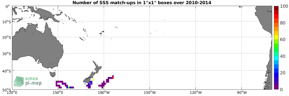
Figure 4: Number of SSS match-ups between Sea mammals SSS and the SMOS SSS L3 v3 Monthly (ICDC) SSS product for the South Pacific Ocean Pi-MEP region over 1^\circ \times 1^\circ boxes and for the full satellite product period.
