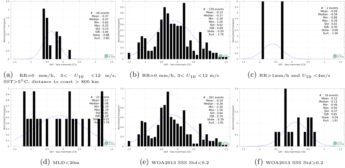
Figure 13: Normalized histogram of \Delta SSS (SMOS SSS L3 v3 Monthly (ICDC) - Sea mammals) for 6 different subdatasets corresponding to: RR=0 mm/h, 3 < U_{10} < 12 m/s, SST > 5^\circ C , distance to coast > 800 km (a), RR=0 mm/h, 3 < U_{10} < 12 m/s (b), RR > 1 mm/h and U_{10} < 4 m/s (c), MLD < 20 m (d), WOA2013 SSS Std < 0.2 (e), WOA2013 SSS Std > 0.2 (f).
