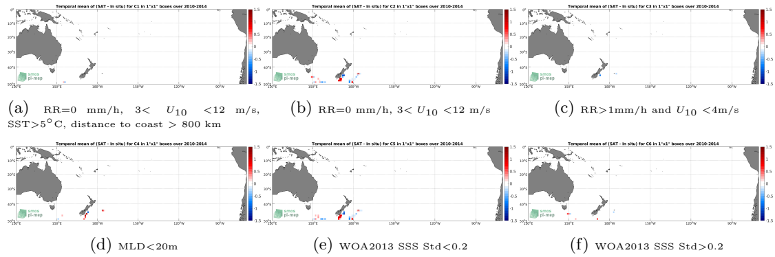
Figure 12: Temporal mean gridded over spatial boxes of size 1^{\circ}\times 1^{\circ} of \Delta\text{SSS} (SMOS SSS L3 v3 Monthly (ICDC) - Sea mammals) for 6 different subdatasets corresponding to: \text{RR}=0 \text{ mm/h} , 3 < U_{10} < 12 \text{ m/s} , \text{SST} > 5^{\circ}\text{C} , distance to coast > 800 \text{ km} (a), \text{RR}=0 \text{ mm/h} , 3 < U_{10} < 12 \text{ m/s} (b), \text{RR} > 1\text{mm/h} and U_{10} < 4\text{m/s} (c), \text{MLD} < 20\text{m} (d), \text{WOA2013 SSS Std} < 0.2 (e), \text{WOA2013 SSS Std} > 0.2 (f).
