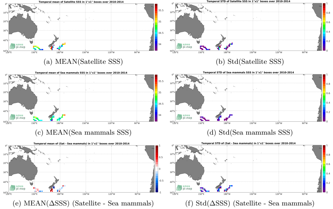
Figure 6: Temporal mean (left) and Std (right) of SSS from SMOS SSS L3 v3 Monthly (ICDC) (top), Sea mammals (middle), and of \Delta SSS (Satellite - Sea mammals). Only match-up pairs are used to generate these maps.
