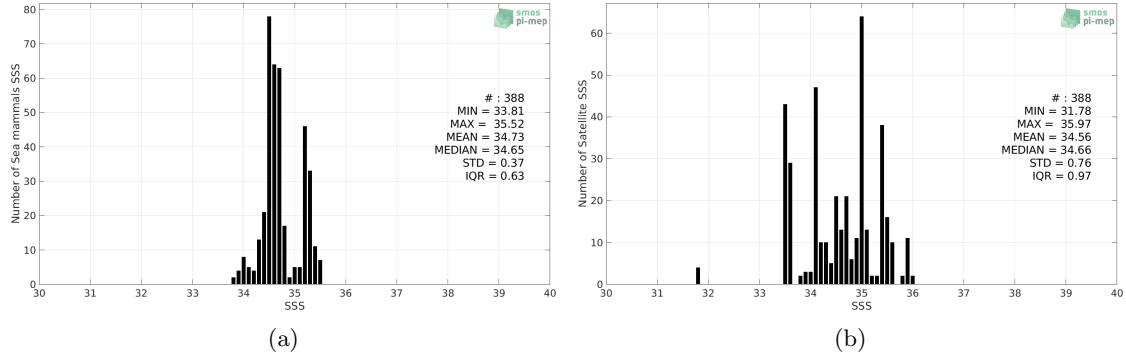
Figure 2: Histograms of SSS from Sea mammals (a) and SMOS SSS L3 v3 Monthly (ICDC) (b) considering all match-up pairs per bins of 0.1 over the South Pacific Ocean Pi-MEP region and for the full satellite product period.
