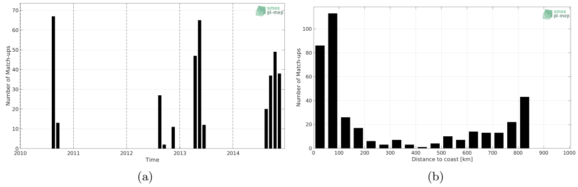
Figure 1: Number of match-ups between Sea mammals and SMOS SSS L3 v3 Monthly (ICDC) SSS as a function of time (a) and as function of the distance to coast (b) over the South Pacific Ocean Pi-MEP region and for the full satellite product period.
