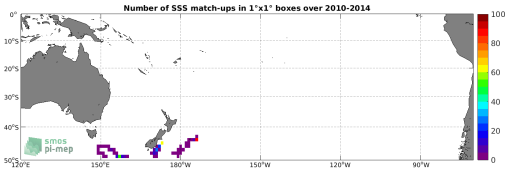
Figure 4: Number of SSS match-ups between Sea mammals SSS and the SMOS SSS L3 v3 Monthly (ICDC) SSS product for the South Pacific Ocean Pi-MEP region over 1°x1° boxes and for the full satellite product period.
