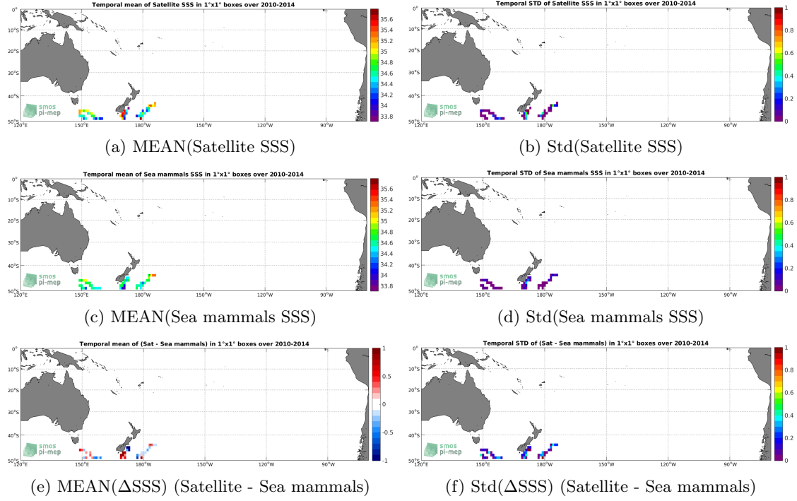
Figure 6: Temporal mean (left) and Std (right) of SSS from SMOS-L3-ICDC-V3-MONTHLY-0.5DEG (top), Sea mammals (middle), and of \Delta SSS (Satellite - Sea mammals). Only match-up pairs are used to generate these maps.
