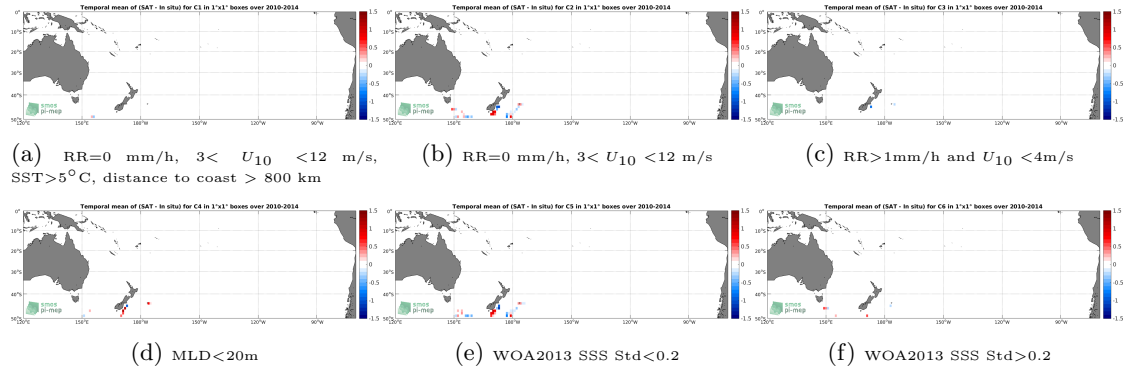
Figure 12: Temporal mean gridded over spatial boxes of size 1^{\circ}\times 1^{\circ} of \Delta\text{SSS} (SMOS-L3-ICDC-V3-MONTHLY-0.5DEG - Sea mammals) for 6 different subdatasets corresponding to:RR=0 mm/h, 3 < U_{10} < 12 m/s, SST >5^{\circ}\text{C} , distance to coast > 800 km (a), RR=0 mm/h, 3 < U_{10} < 12 m/s (b), RR >1\text{mm/h} and U_{10} < 4\text{m/s} (c),MLD <20\text{m} (d),WOA2013 SSS Std <0.2 (e),WOA2013 SSS Std >0.2 (f).
