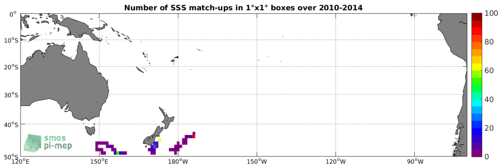
Figure 4: Number of SSS match-ups between Sea mammals SSS and the SMOS-L3-ICDC-V3-MONTHLY-0.5DEG SSS product for the South Pacific Ocean Pi-MEP region over 1^\circ \times 1^\circ boxes and for the full satellite product period.
