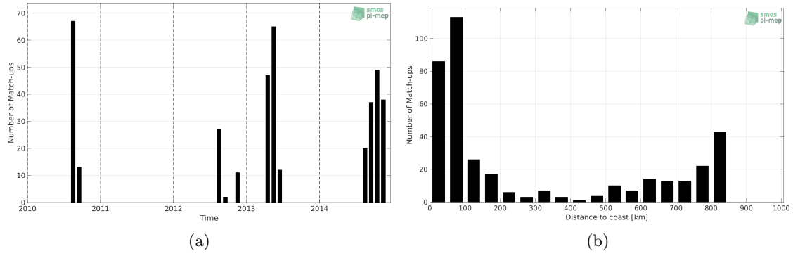
Figure 1: Number of match-ups between Sea mammals and SMOS-L3-ICDC-V3-MONTHLY-0.5DEG SSS as a function of time (a) and as function of the distance to coast (b) over the South Pacific Ocean Pi-MEP region and for the full satellite product period.
