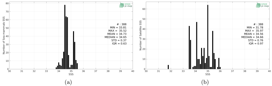
Figure 2: Histograms of SSS from Sea mammals (a) and SMOS-L3-ICDC-V3-MONTHLY-0.5DEG (b) considering all match-up pairs per bins of 0.1 over the South Pacific Ocean Pi-MEP region and for the full satellite product period.
