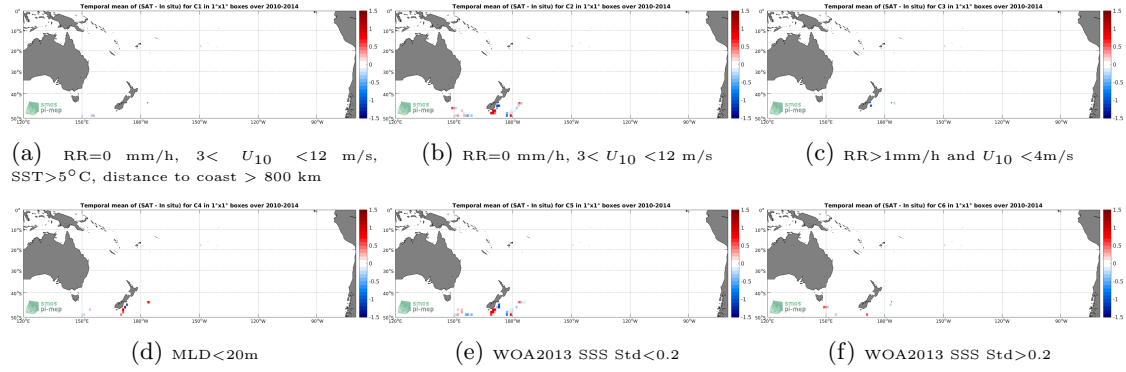
Figure 12: Temporal mean gridded over spatial boxes of size 1^\circ \times 1^\circ of \Delta SSS (SMOS-L3-ICDC-V3-MONTHLY-0.5DEG - Sea mammals) for 6 different subdatasets corresponding to: RR=0 mm/h, 3 < U_{10} < 12 m/s, SST > 5^\circ C , distance to coast > 800 km (a), RR=0 mm/h, 3 < U_{10} < 12 m/s (b), RR > 1 mm/h and U_{10} < 4 m/s (c), MLD < 20 m (d), WOA2013 SSS Std < 0.2 (e), WOA2013 SSS Std > 0.2 (f).
