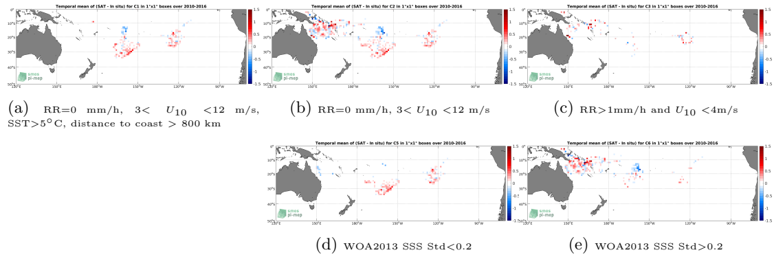
Figure 11: Temporal mean gridded over spatial boxes of size 1^\circ \times 1^\circ of \Delta SSS (SMOS SSS L3 v3 Monthly (ICDC) - Surface drifters) for 5 different subdatasets corresponding to: RR=0 mm/h, 3 < U_{10} < 12 m/s, SST > 5^\circ C , distance to coast > 800 km (a), RR=0 mm/h, 3 < U_{10} < 12 m/s (b), RR > 1 mm/h and U_{10} < 4 m/s (c), WOA2013 SSS Std < 0.2 (d), WOA2013 SSS Std > 0.2 (e).
