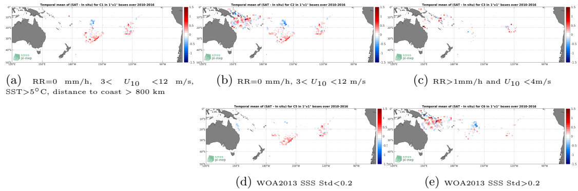
Figure 11: Temporal mean gridded over spatial boxes of size 1^\circ \times 1^\circ of \Delta SSS (SMOS SSS L3 v3 Monthly (ICDC) - Surface drifters) for 5 different subdatasets corresponding to:RR=0 mm/h, 3 < U_{10} < 12 m/s, SST >5^\circ\text{C} , distance to coast > 800 km (a), RR=0 mm/h, 3 < U_{10} < 12 m/s (b), RR >1\text{mm/h} and U_{10} < 4\text{m/s} (c), WOA2013 SSS Std <0.2 (d), WOA2013 SSS Std >0.2 (e).
