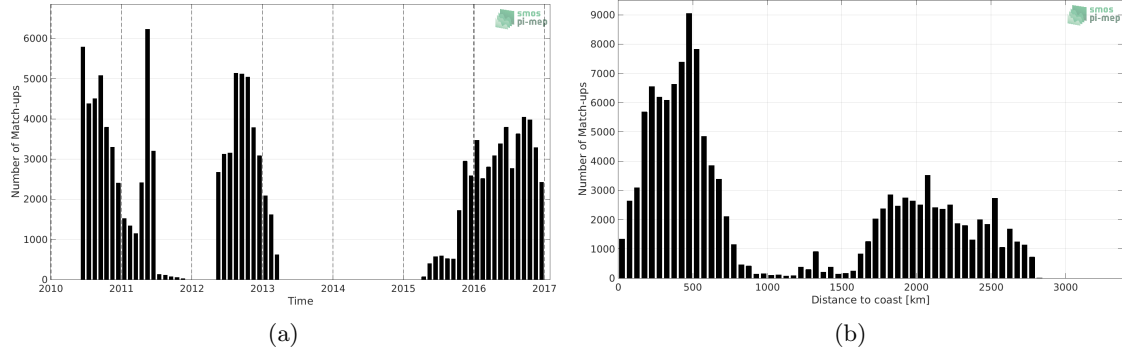
Figure 1: Number of match-ups between Surface drifters and SMOS SSS L3 v3 Monthly (ICDC) SSS as a function of time (a) and as function of the distance to coast (b) over the South Pacific Ocean Pi-MEP region and for the full satellite product period.
