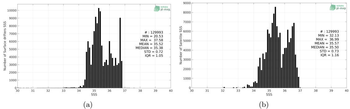
Figure 2: Histograms of SSS from Surface drifters (a) and SMOS SSS L3 v3 Monthly (ICDC) (b) considering all match-up pairs per bins of 0.1 over the South Pacific Ocean Pi-MEP region and for the full satellite product period.
