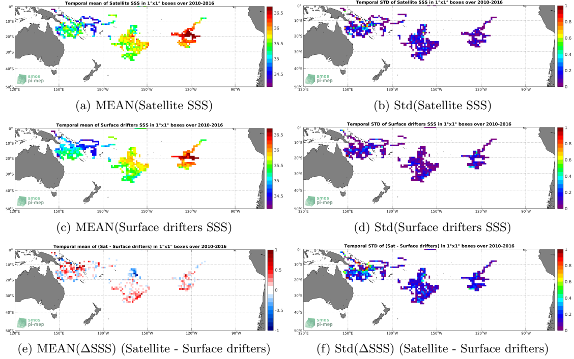
Figure 5: Temporal mean (left) and Std (right) of SSS from SMOS SSS L3 v3 Monthly (ICDC) (top), Surface drifters (middle), and of \Delta SSS (Satellite - Surface drifters). Only match-up pairs are used to generate these maps.
