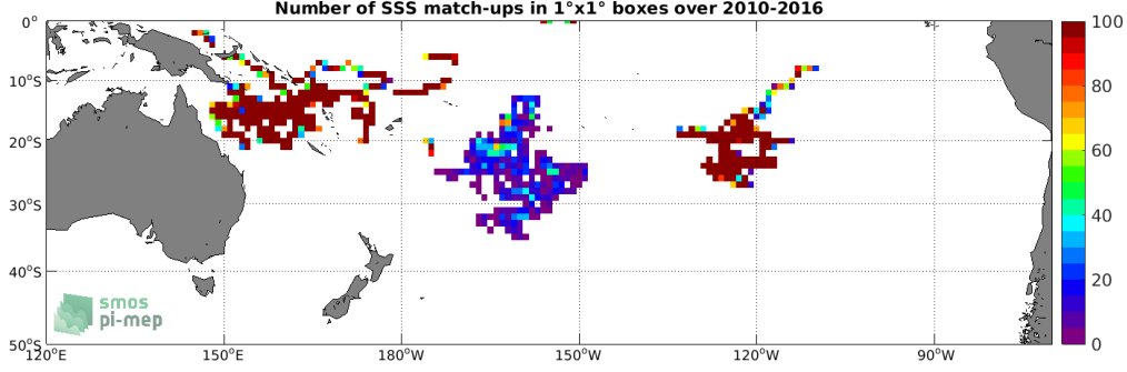
Figure 3: Number of SSS match-ups between Surface drifters SSS and the SMOS SSS L3 v3 Monthly (ICDC) SSS product for the South Pacific Ocean Pi-MEP region over 1^\circ \times 1^\circ boxes and for the full satellite product period.
