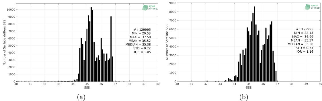
Figure 2: Histograms of SSS from Surface drifters (a) and SMOS-L3-ICDC-V3-MONTHLY-0.5DEG (b) considering all match-up pairs per bins of 0.1 over the South Pacific Ocean Pi-MEP region and for the full satellite product period.
