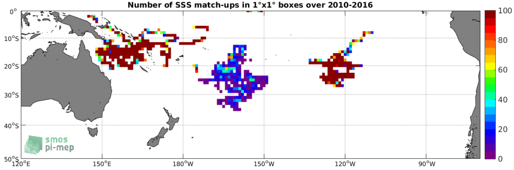
Figure 3: Number of SSS match-ups between Surface drifters SSS and the SMOS-L3-ICDC-V3-MONTHLY-0.5DEG SSS product for the South Pacific Ocean Pi-MEP region over 1^\circ \times 1^\circ boxes and for the full satellite product period.
