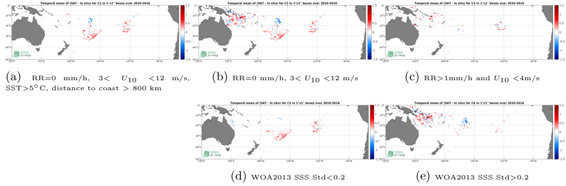
Figure 11: Temporal mean gridded over spatial boxes of size 1^\circ \times 1^\circ of \Delta SSS (SMOS-L3-ICDC-V3-MONTHLY-0.5DEG - Surface drifters) for 5 different subdatasets corresponding to: RR=0 mm/h, 3 < U_{10} < 12 m/s, SST > 5^\circ\text{C} , distance to coast > 800 km (a), RR=0 mm/h, 3 < U_{10} < 12 m/s (b), RR > 1\text{mm/h} and U_{10} < 4\text{m/s} (c), WOA2013 SSS Std < 0.2 (d), WOA2013 SSS Std > 0.2 (e).
