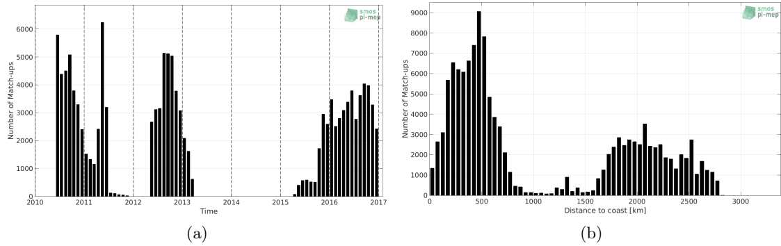
Figure 1: Number of match-ups between Surface drifters and SMOS-L3-ICDC-V3-MONTHLY-0.5DEG SSS as a function of time (a) and as function of the distance to coast (b) over the South Pacific Ocean Pi-MEP region and for the full satellite product period.
