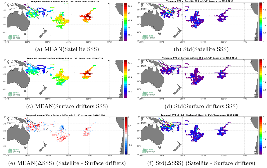
Figure 5: Temporal mean (left) and Std (right) of SSS from SMOS-L3-ICDC-V3-MONTHLY-0.5DEG (top), Surface drifters (middle), and of \Delta SSS (Satellite - Surface drifters). Only match-up pairs are used to generate these maps.
