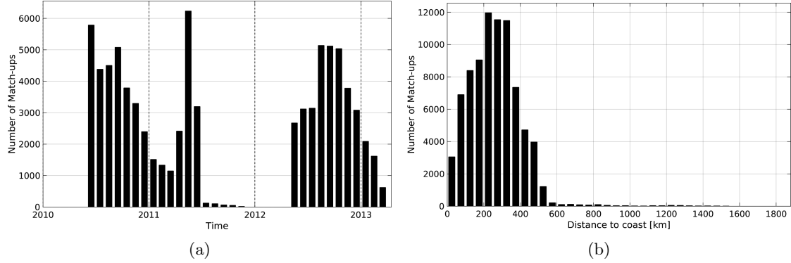
Figure 1: Number of match-ups between Surface drifters and SMOS-L3-ICDC-V3-MONTHLY-0.5DEG SSS as a function of time (a) and as function of the distance to coast (b) over the South Pacific Ocean Pi-MEP region and for the full satellite product period.
