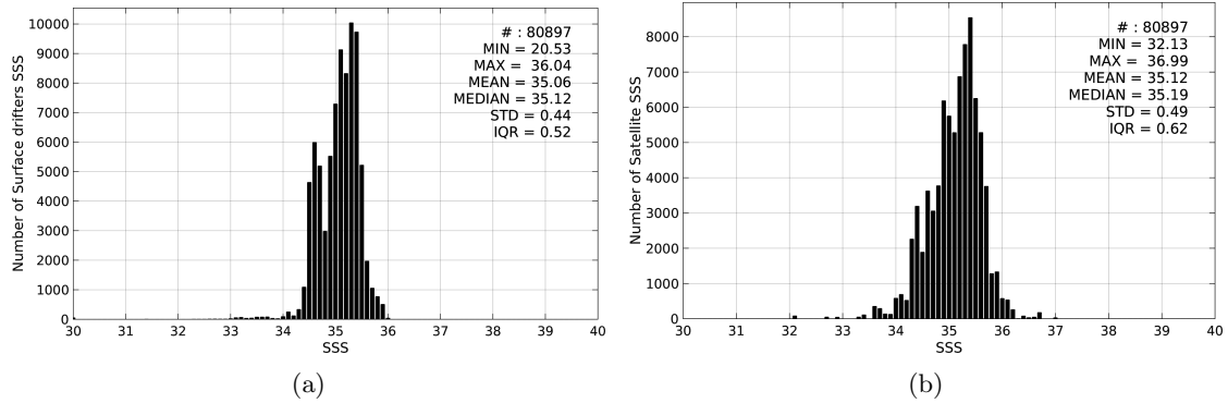
Figure 2: Histograms of SSS from Surface drifters (a) and SMOS-L3-ICDC-V3-MONTHLY-0.5DEG (b) considering all match-up pairs per bins of 0.1 over the South Pacific Ocean Pi-MEP region and for the full satellite product period.
