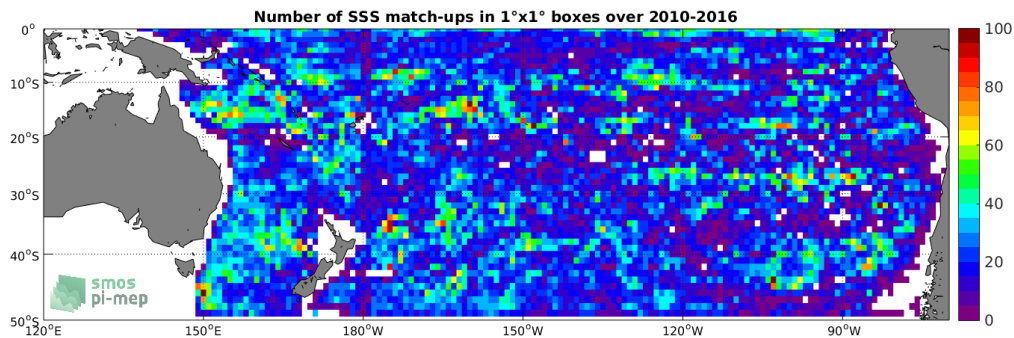
Figure 4: Number of SSS match-ups between Argos SSS and the SMOS-L3-ICDC-V3-MONTHLY-0.5DEG SSS product for the South Pacific Ocean Pi-MEP region over 1^\circ \times 1^\circ boxes and for the full satellite product period.
