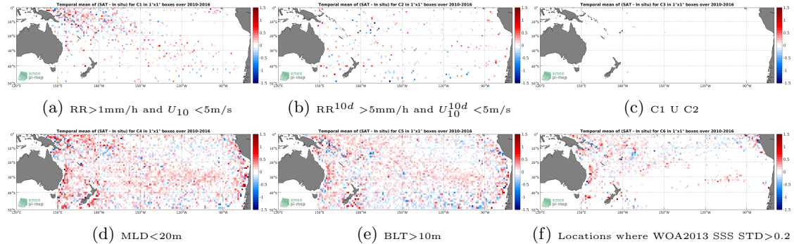
Figure 12: Temporal mean gridded over spatial boxes of size 1^\circ \times 1^\circ of \Delta SSS (SMOS-L3-ICDC-V3-MONTHLY-0.5DEG - Argo) for 6 different subdatasets corresponding to:RR>1mm/h and U_{10} < 5m/s (a), RR^{10d} > 5mm/h and U_{10}^{10d} < 5m/s (b), C1 U C2 (c),MLD<20m (d),BLT>10m (e),Locations where WOA2013 SSS STD>0.2 (f).
