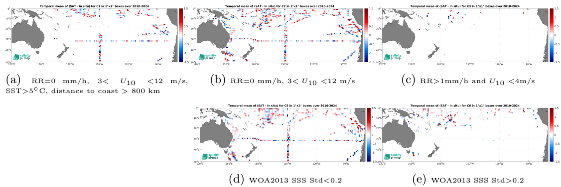
Figure 14: Temporal mean gridded over spatial boxes of size 1^\circ \times 1^\circ of \Delta SSS (SMOS SSS L2Q v331 - With FLAG (CMEMS-CATDS-CPDC) - TSG (SAMOS)) for 5 different subdatasets corresponding to:RR=0 mm/h, 3 < U_{10} < 12 m/s, SST>5°C, distance to coast > 800 km (a), RR=0 mm/h, 3 < U_{10} < 12 m/s (b), RR>1mm/h and U_{10} < 4 m/s (c), WOA2013 SSS Std<0.2 (d), WOA2013 SSS Std>0.2 (e).
