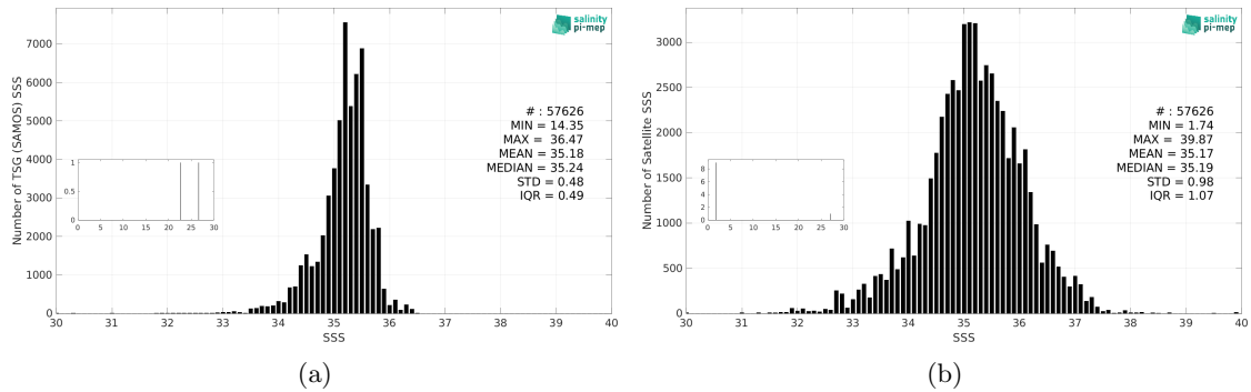
Figure 3: Histograms of SSS from TSG (SAMOS) (a) and SMOS SSS L2Q v331 - With FLAG (CMEMS-CATDS-CPDC) (b) considering all match-up pairs per bins of 0.1 over the South Pacific Ocean Pi-MEP region and for the full satellite product period.
