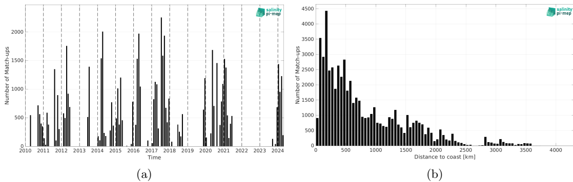
Figure 2: Number of match-ups between TSG (SAMOS) and SMOS SSS L2Q v331 - With FLAG (CMEMS-CATDS-CPDC) SSS as a function of time (a) and as function of the distance to coast (b) over the South Pacific Ocean Pi-MEP region and for the full satellite product period.
