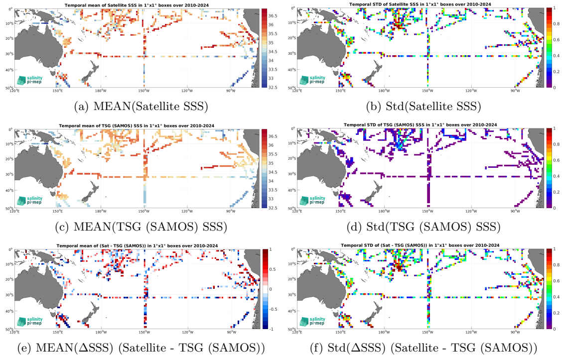
Figure 7: Temporal mean (left) and Std (right) of SSS from SMOS SSS L2Q v331 - With FLAG (CMEMS-CATDS-CPDC) (top), TSG (SAMOS) (middle), and of \Delta SSS (Satellite - TSG (SAMOS)). Only match-up pairs are used to generate these maps.
