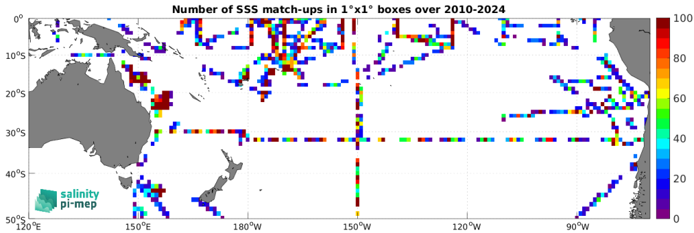
Figure 5: Number of SSS match-ups between TSG (SAMOS) SSS and the SMOS SSS L2Q v331 - With FLAG (CMEMS-CATDS-CPDC) SSS product for the South Pacific Ocean Pi-MEP region over 1^\circ \times 1^\circ boxes and for the full satellite product period.
