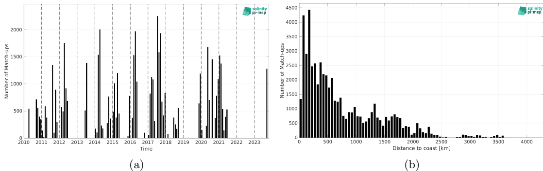
Figure 1: Number of match-ups between TSG (SAMOS) and SMOS SSS L2Q v331 - With FLAG (CMEMS-CATDS-CPDC) SSS as a function of time (a) and as function of the distance to coast (b) over the South Pacific Ocean Pi-MEP region and for the full satellite product period.
