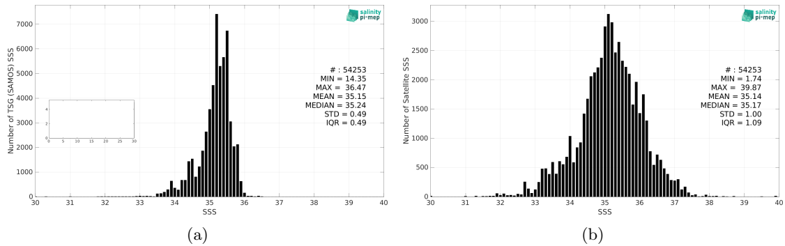
Figure 2: Histograms of SSS from TSG (SAMOS) (a) and SMOS SSS L2Q v331 - With FLAG (CMEMS-CATDS-CPDC) (b) considering all match-up pairs per bins of 0.1 over the South Pacific Ocean Pi-MEP region and for the full satellite product period.
