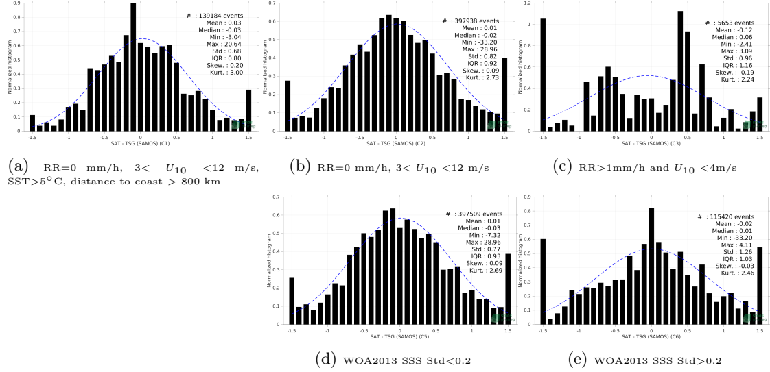
Figure 13: Normalized histogram of \Delta SSS (SMOS SSS L2Q v331 - With FLAG (CMEMS-CATDS-CPDC) - TSG (SAMOS)) for 5 different subdatasets corresponding to: RR=0 mm/h, 3 < U_{10} < 12 m/s, SST > 5°C, distance to coast > 800 km (a), RR=0 mm/h, 3 < U_{10} < 12 m/s (b), RR > 1mm/h and U_{10} < 4 m/s (c), WOA2013 SSS Std < 0.2 (d), WOA2013 SSS Std > 0.2 (e).
