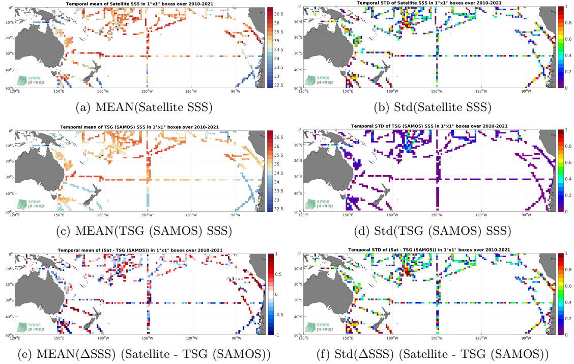
Figure 6: Temporal mean (left) and Std (right) of SSS from SMOS SSS L2Q v331 - With FLAG (CMEMS-CATDS-CPDC) (top), TSG (SAMOS) (middle), and of \Delta SSS (Satellite - TSG (SAMOS)). Only match-up pairs are used to generate these maps.
