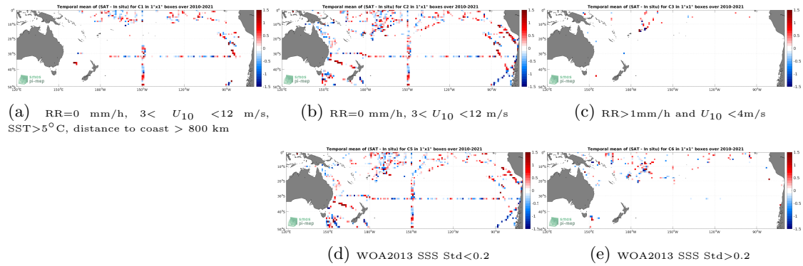
Figure 12: Temporal mean gridded over spatial boxes of size 1^\circ \times 1^\circ of \Delta SSS (SMOS SSS L2Q v331 - With FLAG (CMEMS-CATDS-CPDC) - TSG (SAMOS)) for 5 different subdatasets corresponding to:RR=0 mm/h, 3 < U_{10} < 12 m/s, SST >5^\circ C, distance to coast > 800 km (a), RR=0 mm/h, 3 < U_{10} < 12 m/s (b), RR >1 mm/h and U_{10} < 4 m/s (c), WOA2013 SSS Std <0.2 (d), WOA2013 SSS Std >0.2 (e).
