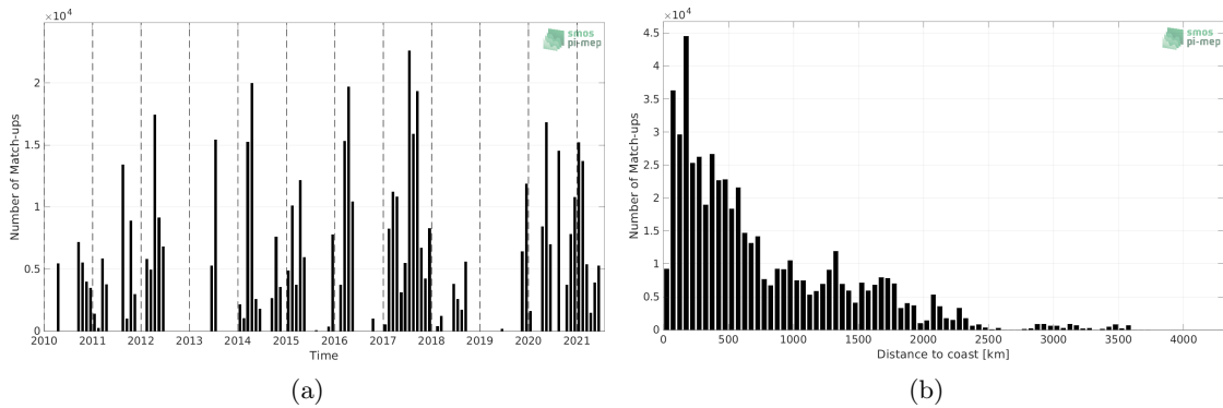
Figure 1: Number of match-ups between TSG (SAMOS) and SMOS SSS L2Q v331 - With FLAG (CMEMS-CATDS-CPDC) SSS as a function of time (a) and as function of the distance to coast (b) over the South Pacific Ocean Pi-MEP region and for the full satellite product period.
