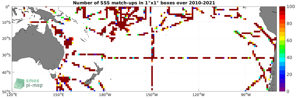
Figure 4: Number of SSS match-ups between TSG (SAMOS) SSS and the SMOS SSS L2Q v331 - With FLAG (CMEMS-CATDS-CPDC) SSS product for the South Pacific Ocean Pi-MEP region over 1^\circ \times 1^\circ boxes and for the full satellite product period.
