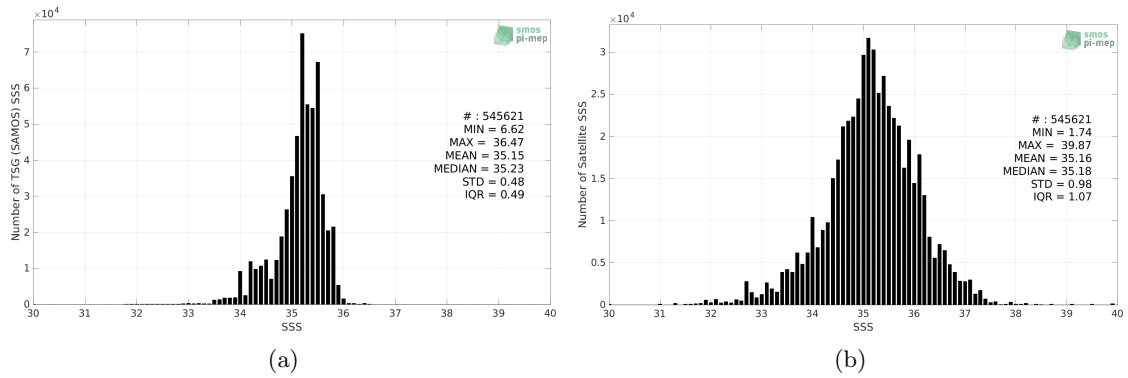
Figure 2: Histograms of SSS from TSG (SAMOS) (a) and SMOS SSS L2Q v331 - With FLAG (CMEMS-CATDS-CPDC) (b) considering all match-up pairs per bins of 0.1 over the South Pacific Ocean Pi-MEP region and for the full satellite product period.
