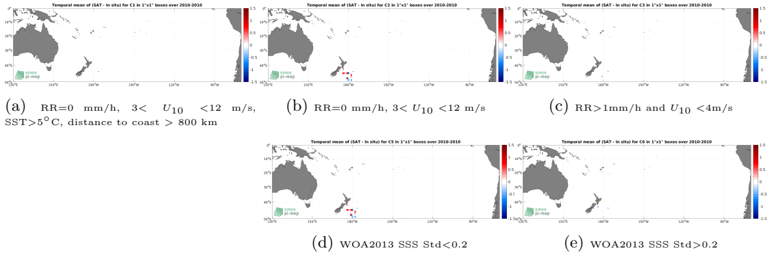
Figure 12: Temporal mean gridded over spatial boxes of size 1^{\circ}\times 1^{\circ} of \Delta\text{SSS} (SMOS SSS L2Q v331 - With FLAG (CMEMS-CATDS-CPDC) - TSG (Polarstern)) for 5 different subdatasets corresponding to:RR=0 mm/h, 3 < U_{10} < 12 m/s, SST >5^{\circ}\text{C} , distance to coast > 800 km (a), RR=0 mm/h, 3 < U_{10} < 12 m/s (b), RR >1 mm/h and U_{10} < 4 m/s (c), WOA2013 SSS Std <0.2 (d), WOA2013 SSS Std >0.2 (e).
