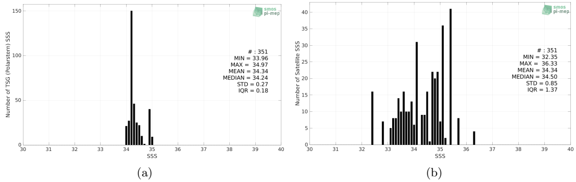
Figure 2: Histograms of SSS from TSG (Polarstern) (a) and SMOS SSS L2Q v331 - With FLAG (CMEMS-CATDS-CPDC) (b) considering all match-up pairs per bins of 0.1 over the South Pacific Ocean Pi-MEP region and for the full satellite product period.
