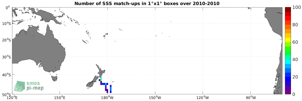
Figure 4: Number of SSS match-ups between TSG (Polarstern) SSS and the SMOS SSS L2Q v331 - With FLAG (CMEMS-CATDS-CPDC) SSS product for the South Pacific Ocean Pi-MEP region over 1^\circ \times 1^\circ boxes and for the full satellite product period.
