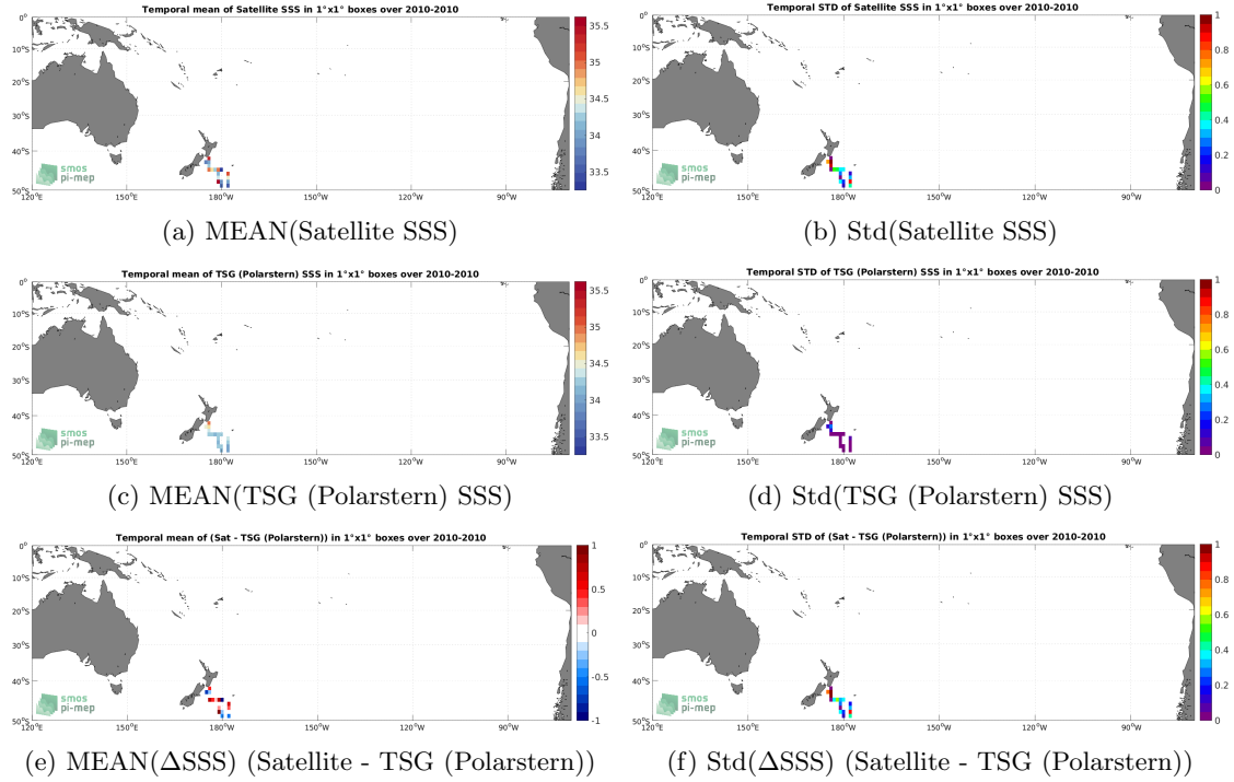
Figure 6: Temporal mean (left) and Std (right) of SSS from SMOS SSS L2Q v331 - With FLAG (CMEMS-CATDS-CPDC) (top), TSG (Polarstern) (middle), and of \Delta SSS (Satellite - TSG (Polarstern)). Only match-up pairs are used to generate these maps.
