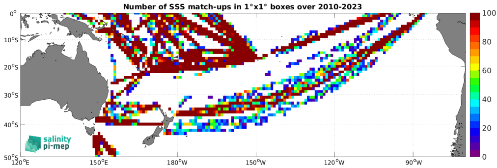
Figure 5: Number of SSS match-ups between TSG (LEGOS-DM) SSS and the SMOS SSS L2Q v331 - With FLAG (CMEMS-CATDS-CPDC) SSS product for the South Pacific Ocean Pi-MEP region over 1^\circ \times 1^\circ boxes and for the full satellite product period.
