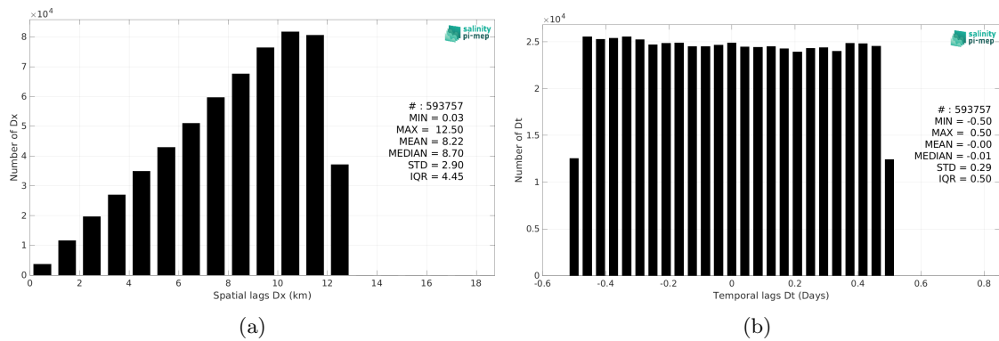
Figure 6: Histograms of the spatial (a) and temporal (b) lags between the location/time of the TSG (LEGOS-DM) measurement and the date of the corresponding SMOS SSS L2Q v331 - With FLAG (CMEMS-CATDS-CPDC) SSS pixel.
