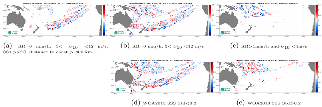
Figure 14: Temporal mean gridded over spatial boxes of size 1^\circ \times 1^\circ of \Delta\text{SSS} (SMOS SSS L2Q v331 - With FLAG (CMEMS-CATDS-CPDC) - TSG (LEGOS-DM)) for 5 different subdatasets corresponding to:RR=0 mm/h, 3 < U_{10} < 12 m/s, SST>5°C, distance to coast > 800 km (a), RR=0 mm/h, 3 < U_{10} < 12 m/s (b), RR>1mm/h and U_{10} < 4 m/s (c), WOA2013 SSS Std<0.2 (d), WOA2013 SSS Std>0.2 (e).
