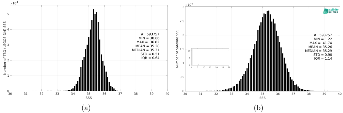
Figure 3: Histograms of SSS from TSG (LEGOS-DM) (a) and SMOS SSS L2Q v331 - With FLAG (CMEMS-CATDS-CPDC) (b) considering all match-up pairs per bins of 0.1 over the South Pacific Ocean Pi-MEP region and for the full satellite product period.
