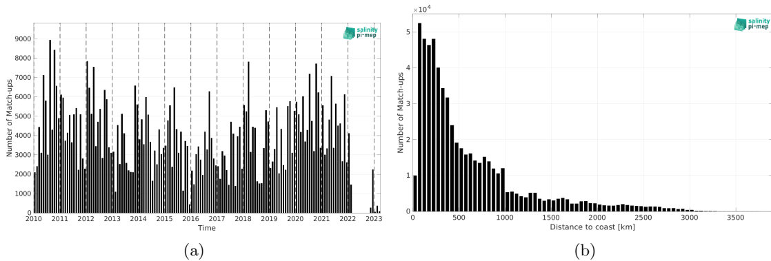
Figure 2: Number of match-ups between TSG (LEGOS-DM) and SMOS SSS L2Q v331 - With FLAG (CMEMS-CATDS-CPDC) SSS as a function of time (a) and as function of the distance to coast (b) over the South Pacific Ocean Pi-MEP region and for the full satellite product period.
