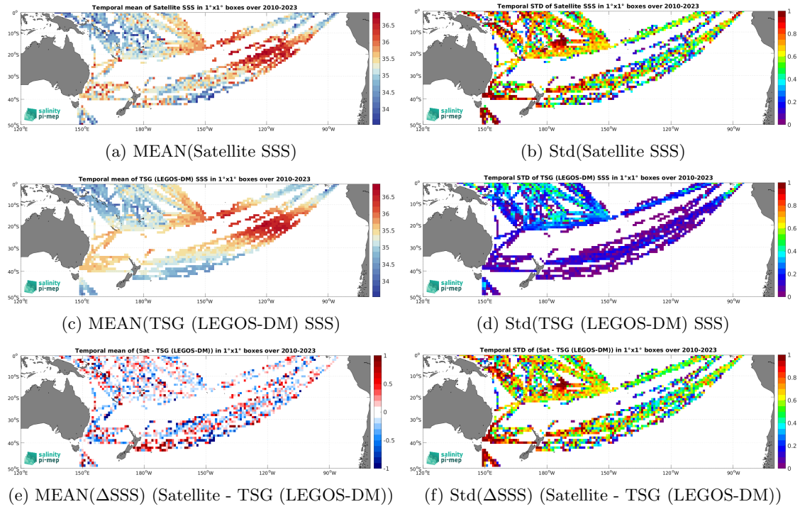
Figure 7: Temporal mean (left) and Std (right) of SSS from SMOS SSS L2Q v331 - With FLAG (CMEMS-CATDS-CPDC) (top), TSG (LEGOS-DM) (middle), and of \Delta SSS (Satellite - TSG (LEGOS-DM)). Only match-up pairs are used to generate these maps.
