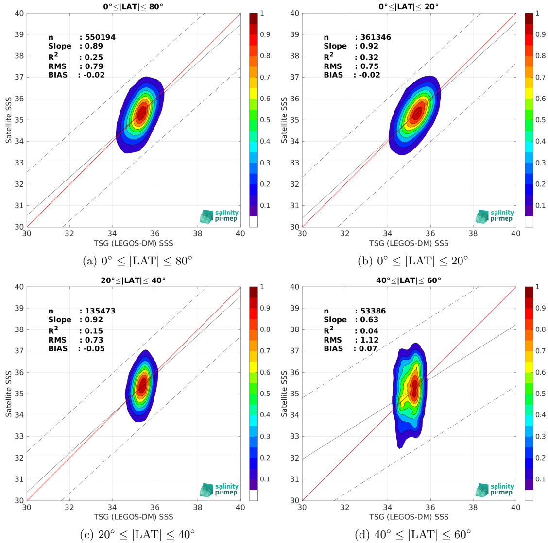
Figure 9: Contour maps of the concentration of SMOS SSS L2Q v331 - With FLAG (CMEMS-CATDS-CPDC) SSS ( y -axis) versus TSG (LEGOS-DM) SSS ( x -axis) at match-up pairs for different latitude bands. For each plot, the red line shows x=y . The black thin and dashed lines indicate a linear fit through the data cloud and the \pm 95\% confidence levels, respectively. The number match-up pairs n , the slope and R^2 coefficient of the linear fit, the root mean square (RMS) and the mean bias between satellite and in situ data are indicated for each latitude band in each plots.
