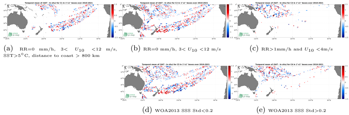
Figure 12: Temporal mean gridded over spatial boxes of size 1^\circ \times 1^\circ of \Delta SSS (SMOS SSS L2Q v331 - With FLAG (CMEMS-CATDS-CPDC) - TSG (LEGOS-DM)) for 5 different subdatasets corresponding to:RR=0 mm/h, 3 < U_{10} < 12 m/s, SST >5^\circ\text{C} , distance to coast > 800 km (a), RR=0 mm/h, 3 < U_{10} < 12 m/s (b), RR >1 mm/h and U_{10} < 4 m/s (c), WOA2013 SSS Std <0.2 (d), WOA2013 SSS Std >0.2 (e).
