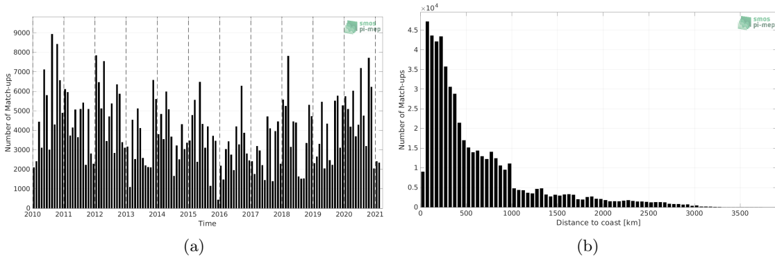
Figure 1: Number of match-ups between TSG (LEGOS-DM) and SMOS SSS L2Q v331 - With FLAG (CMEMS-CATDS-CPDC) SSS as a function of time (a) and as function of the distance to coast (b) over the South Pacific Ocean Pi-MEP region and for the full satellite product period.
