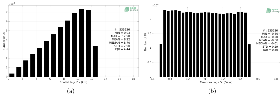
Figure 5: Histograms of the spatial (a) and temporal (b) lags between the location/time of the TSG (LEGOS-DM) measurement and the date of the corresponding SMOS SSS L2Q v331 - With FLAG (CMEMS-CATDS-CPDC) SSS pixel.
