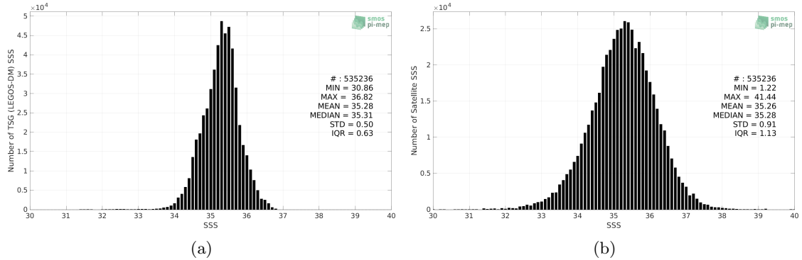
Figure 2: Histograms of SSS from TSG (LEGOS-DM) (a) and SMOS SSS L2Q v331 - With FLAG (CMEMS-CATDS-CPDC) (b) considering all match-up pairs per bins of 0.1 over the South Pacific Ocean Pi-MEP region and for the full satellite product period.
