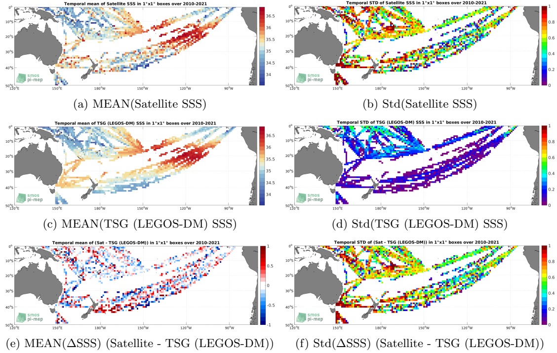
Figure 6: Temporal mean (left) and Std (right) of SSS from SMOS SSS L2Q v331 - With FLAG (CMEMS-CATDS-CPDC) (top), TSG (LEGOS-DM) (middle), and of \Delta SSS (Satellite - TSG (LEGOS-DM)). Only match-up pairs are used to generate these maps.
