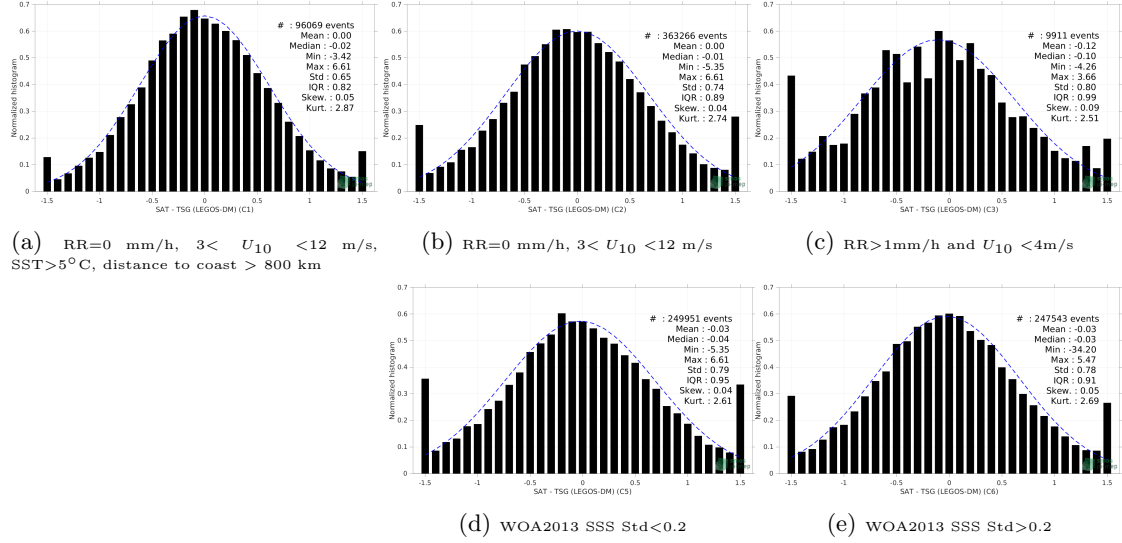
Figure 13: Normalized histogram of \Delta\text{SSS} (SMOS SSS L2Q v331 - With FLAG (CMEMS-CATDS-CPDC) - TSG (LEGOS-DM)) for 5 different subdatasets corresponding to: RR=0 mm/h, 3 < U_{10} < 12 m/s, SST > 5^\circ\text{C} , distance to coast > 800 km (a), RR=0 mm/h, 3 < U_{10} < 12 m/s (b), RR > 1 mm/h and U_{10} < 4 m/s (c), WOA2013 SSS Std < 0.2 (d), WOA2013 SSS Std > 0.2 (e).
