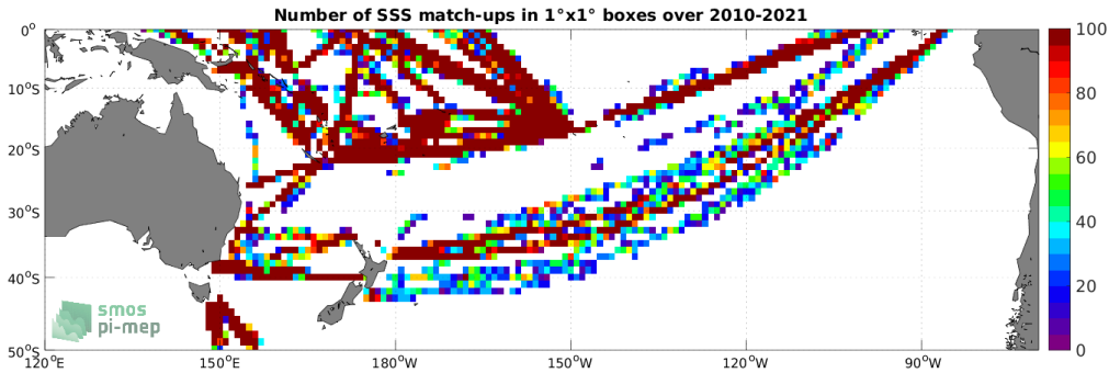
Figure 4: Number of SSS match-ups between TSG (LEGOS-DM) SSS and the SMOS SSS L2Q v331 - With FLAG (CMEMS-CATDS-CPDC) SSS product for the South Pacific Ocean Pi-MEP region over 1^\circ \times 1^\circ boxes and for the full satellite product period.
