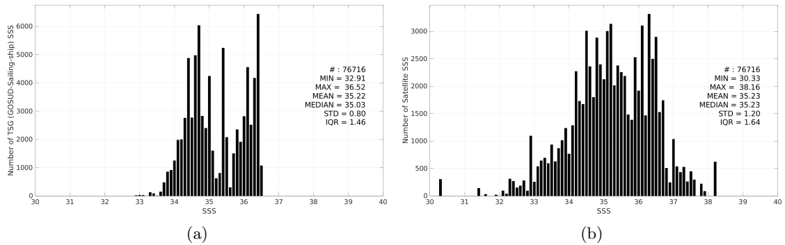
Figure 3: Histograms of SSS from TSG (GOSUD-Sailing-ship) (a) and SMOS SSS L2Q v331 - With FLAG (CMEMS-CATDS-CPDC) (b) considering all match-up pairs per bins of 0.1 over the South Pacific Ocean Pi-MEP region and for the full satellite product period.
