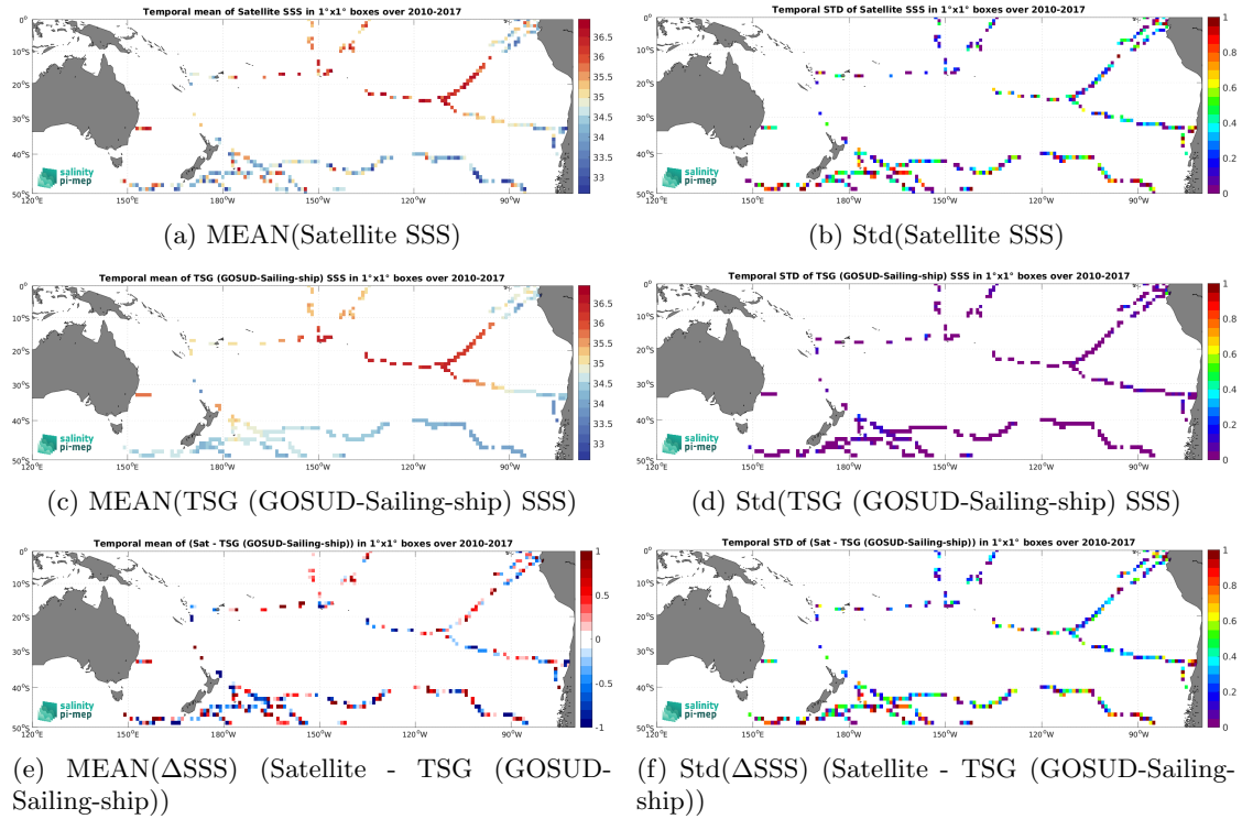
Figure 7: Temporal mean (left) and Std (right) of SSS from SMOS SSS L2Q v331 - With FLAG (CMEMS-CATDS-CPDC) (top), TSG (GOSUD-Sailing-ship) (middle), and of \Delta SSS (Satellite - TSG (GOSUD-Sailing-ship)). Only match-up pairs are used to generate these maps.
