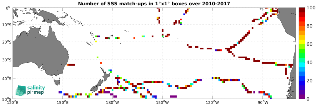
Figure 5: Number of SSS match-ups between TSG (GOSUD-Sailing-ship) SSS and the SMOS SSS L2Q v331 - With FLAG (CMEMS-CATDS-CPDC) SSS product for the South Pacific Ocean Pi-MEP region over 1^\circ \times 1^\circ boxes and for the full satellite product period.
