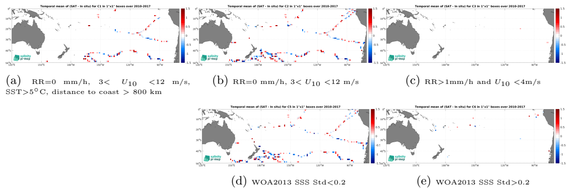
Figure 14: Temporal mean gridded over spatial boxes of size 1^\circ \times 1^\circ of \Delta\text{SSS} (SMOS SSS L2Q v331 - With FLAG (CMEMS-CATDS-CPDC) - TSG (GOSUD-Sailing-ship)) for 5 different subdatasets corresponding to:RR=0 mm/h, 3 < U_{10} < 12 m/s, SST>5°C, distance to coast > 800 km (a), RR=0 mm/h, 3 < U_{10} < 12 m/s (b), RR>1mm/h and U_{10} < 4 m/s (c), WOA2013 SSS Std<0.2 (d), WOA2013 SSS Std>0.2 (e).
