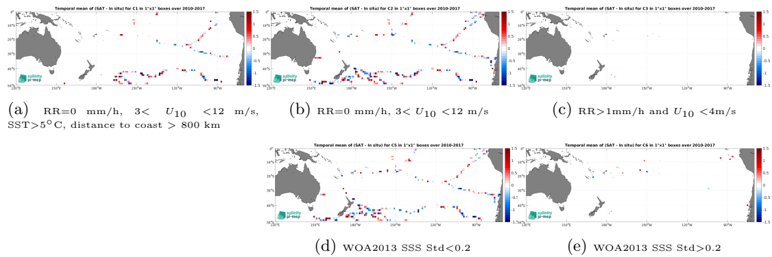
Figure 12: Temporal mean gridded over spatial boxes of size 1^\circ \times 1^\circ of \Delta SSS (SMOS SSS L2Q v331 - With FLAG (CMEMS-CATDS-CPDC) - TSG (GOSUD-Sailing-ship)) for 5 different subdatasets corresponding to:RR=0 mm/h, 3 < U_{10} < 12 m/s, SST>5°C, distance to coast > 800 km (a), RR=0 mm/h, 3 < U_{10} < 12 m/s (b), RR>1mm/h and U_{10} < 4 m/s (c), WOA2013 SSS Std<0.2 (d), WOA2013 SSS Std>0.2 (e).
