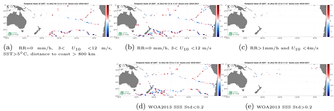
Figure 12: Temporal mean gridded over spatial boxes of size 1^\circ \times 1^\circ of \Delta\text{SSS} (SMOS SSS L2Q v331 - With FLAG (CMEMS-CATDS-CPDC) - TSG (GOSUD-Sailing-ship)) for 5 different subdatasets corresponding to:RR=0 mm/h, 3 < U_{10} < 12 m/s, SST>5°C, distance to coast > 800 km (a), RR=0 mm/h, 3 < U_{10} < 12 m/s (b), RR>1mm/h and U_{10} < 4 m/s (c), WOA2013 SSS Std<0.2 (d), WOA2013 SSS Std>0.2 (e).
