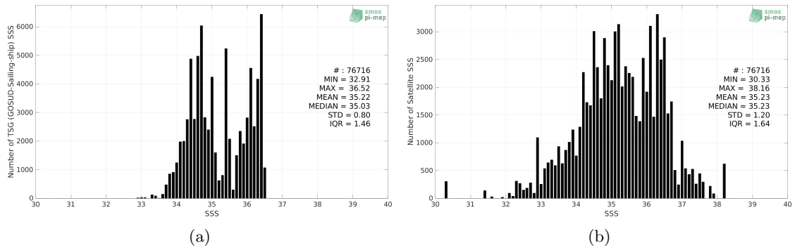
Figure 2: Histograms of SSS from TSG (GOSUD-Sailing-ship) (a) and SMOS SSS L2Q v331 - With FLAG (CMEMS-CATDS-CPDC) (b) considering all match-up pairs per bins of 0.1 over the South Pacific Ocean Pi-MEP region and for the full satellite product period.
