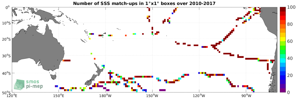
Figure 4: Number of SSS match-ups between TSG (GOSUD-Sailing-ship) SSS and the SMOS SSS L2Q v331 - With FLAG (CMEMS-CATDS-CPDC) SSS product for the South Pacific Ocean Pi-MEP region over 1^\circ \times 1^\circ boxes and for the full satellite product period.
