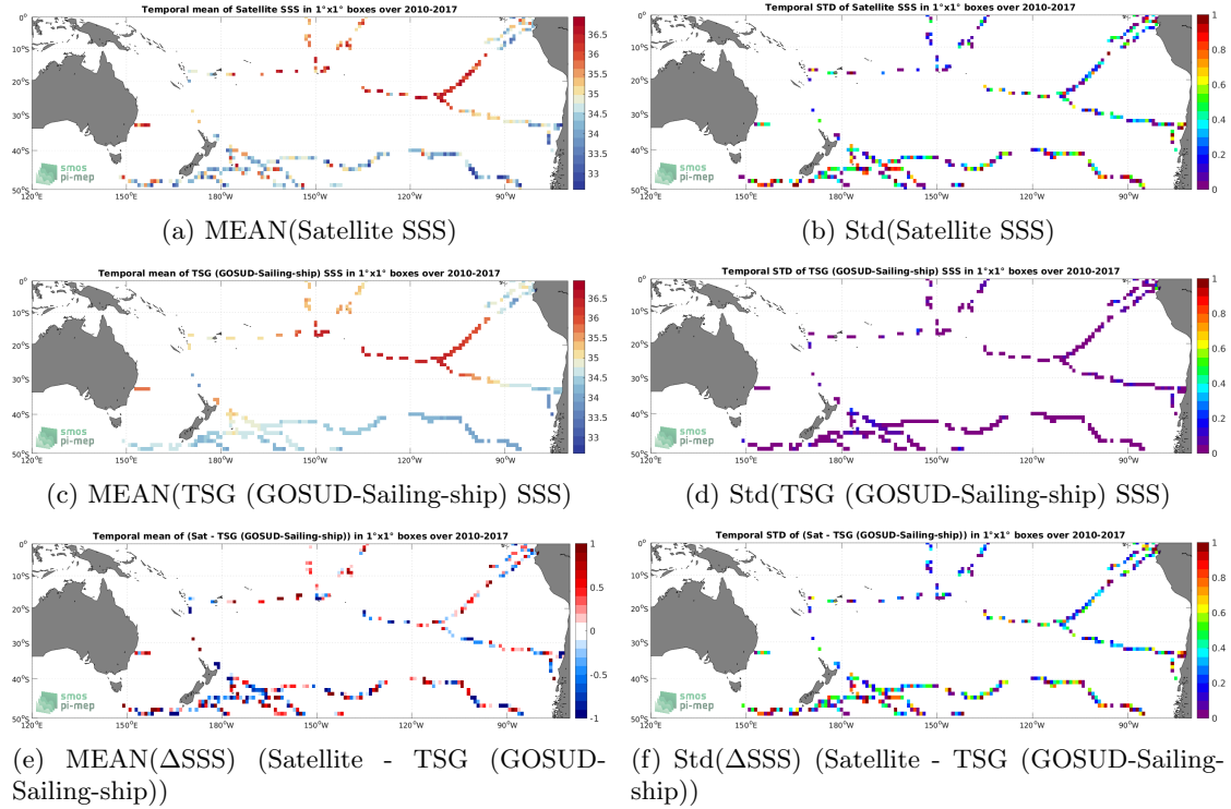
Figure 6: Temporal mean (left) and Std (right) of SSS from SMOS SSS L2Q v331 - With FLAG (CMEMS-CATDS-CPDC) (top), TSG (GOSUD-Sailing-ship) (middle), and of \Delta SSS (Satellite - TSG (GOSUD-Sailing-ship)). Only match-up pairs are used to generate these maps.
