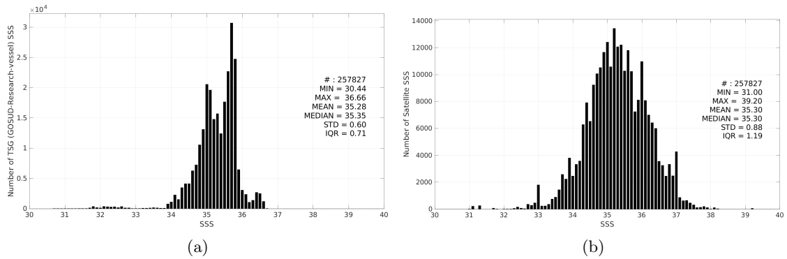
Figure 3: Histograms of SSS from TSG (GOSUD-Research-vessel) (a) and SMOS SSS L2Q v331 - With FLAG (CMEMS-CATDS-CPDC) (b) considering all match-up pairs per bins of 0.1 over the South Pacific Ocean Pi-MEP region and for the full satellite product period.
