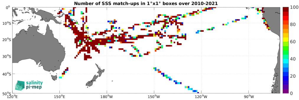
Figure 5: Number of SSS match-ups between TSG (GOSUD-Research-vessel) SSS and the SMOS SSS L2Q v331 - With FLAG (CMEMS-CATDS-CPDC) SSS product for the South Pacific Ocean Pi-MEP region over 1^\circ \times 1^\circ boxes and for the full satellite product period.
