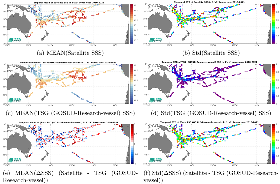
Figure 7: Temporal mean (left) and Std (right) of SSS from SMOS SSS L2Q v331 - With FLAG (CMEMS-CATDS-CPDC) (top), TSG (GOSUD-Research-vessel) (middle), and of \Delta SSS (Satellite - TSG (GOSUD-Research-vessel)). Only match-up pairs are used to generate these maps.
