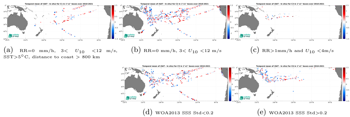
Figure 14: Temporal mean gridded over spatial boxes of size 1^\circ \times 1^\circ of \Delta\text{SSS} (SMOS SSS L2Q v331 - With FLAG (CMEMS-CATDS-CPDC) - TSG (GOSUD-Research-vessel)) for 5 different subdatasets corresponding to:RR=0 mm/h, 3 < U_{10} < 12 m/s, SST >5^\circ\text{C} , distance to coast > 800 km (a), RR=0 mm/h, 3 < U_{10} < 12 m/s (b), RR >1 mm/h and U_{10} < 4 m/s (c), WOA2013 SSS Std <0.2 (d), WOA2013 SSS Std >0.2 (e).
