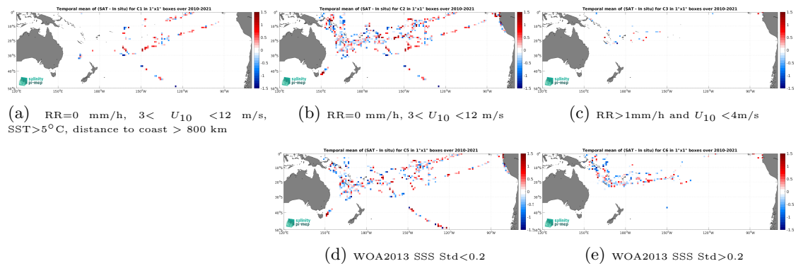
Figure 12: Temporal mean gridded over spatial boxes of size 1^\circ \times 1^\circ of \Delta\text{SSS} (SMOS SSS L2Q v331 - With FLAG (CMEMS-CATDS-CPDC) - TSG (GOSUD-Research-vessel)) for 5 different subdatasets corresponding to:RR=0 mm/h, 3 < U_{10} < 12 m/s, SST >5^\circ\text{C} , distance to coast > 800 km (a), RR=0 mm/h, 3 < U_{10} < 12 m/s (b), RR >1 mm/h and U_{10} < 4 m/s (c), WOA2013 SSS Std <0.2 (d), WOA2013 SSS Std >0.2 (e).
