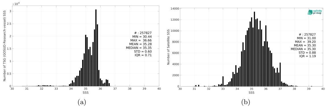
Figure 2: Histograms of SSS from TSG (GOSUD-Research-vessel) (a) and SMOS SSS L2Q v331 - With FLAG (CMEMS-CATDS-CPDC) (b) considering all match-up pairs per bins of 0.1 over the South Pacific Ocean Pi-MEP region and for the full satellite product period.
