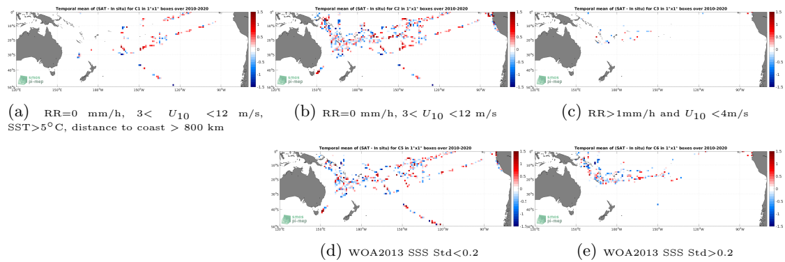
Figure 12: Temporal mean gridded over spatial boxes of size 1^\circ \times 1^\circ of \Delta SSS (SMOS SSS L2Q v331 - With FLAG (CMEMS-CATDS-CPDC) - TSG (GOSUD-Research-vessel)) for 5 different subdatasets corresponding to:RR=0 mm/h, 3 < U_{10} < 12 m/s, SST >5^\circ C, distance to coast > 800 km (a), RR=0 mm/h, 3 < U_{10} < 12 m/s (b), RR >1 mm/h and U_{10} < 4 m/s (c), WOA2013 SSS Std <0.2 (d), WOA2013 SSS Std >0.2 (e).
