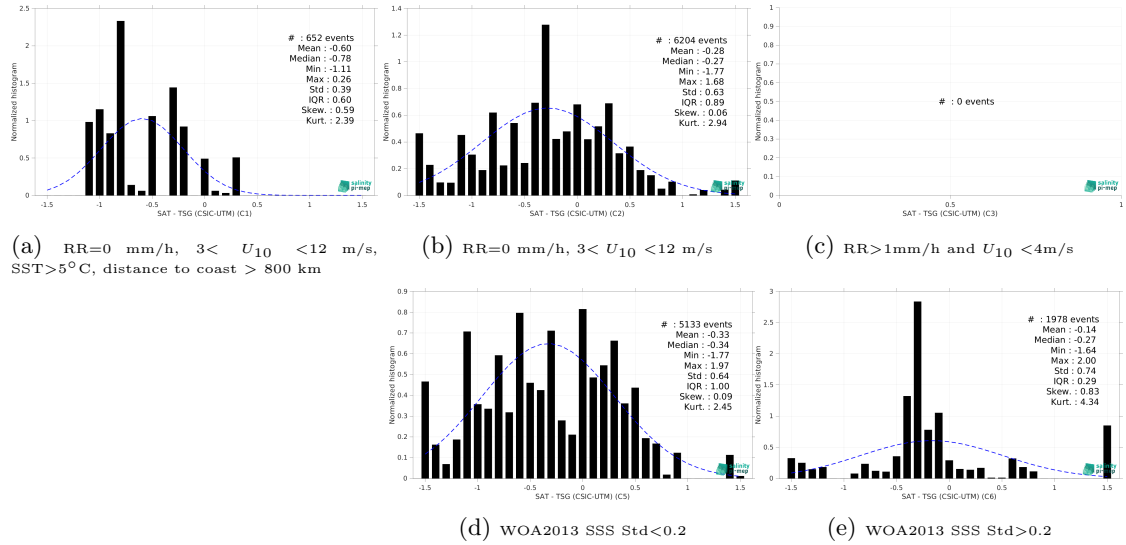
Figure 15: Normalized histogram of \Delta SSS (SMOS SSS L2Q v331 - With FLAG (CMEMS-CATDS-CPDC) - TSG (CSIC-UTM)) for 5 different subdatasets corresponding to: RR=0 mm/h, 3 < U_{10} < 12 m/s, SST>5°C, distance to coast > 800 km (a), RR=0 mm/h, 3 < U_{10} < 12 m/s (b), RR>1mm/h and U_{10} < 4 m/s (c), WOA2013 SSS Std<0.2 (d), WOA2013 SSS Std>0.2 (e).
