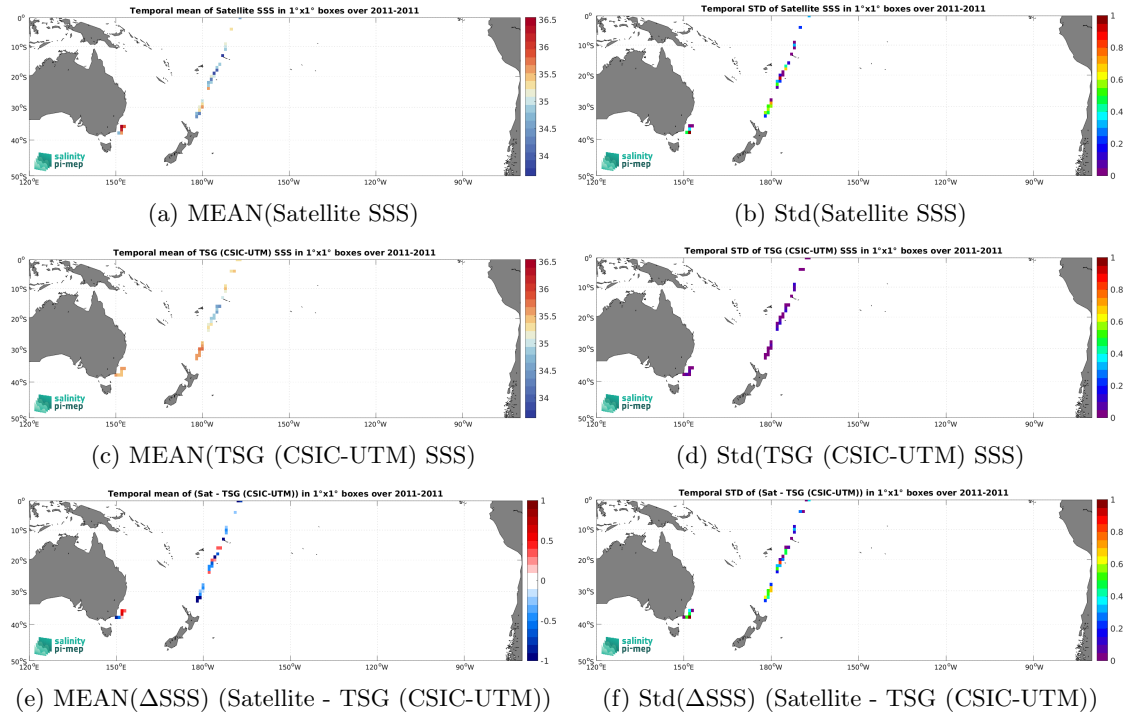
Figure 7: Temporal mean (left) and Std (right) of SSS from SMOS SSS L2Q v331 - With FLAG (CMEMS-CATDS-CPDC) (top), TSG (CSIC-UTM) (middle), and of \Delta SSS (Satellite - TSG (CSIC-UTM)). Only match-up pairs are used to generate these maps.
