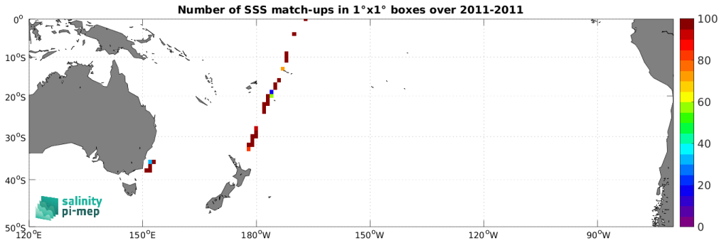
Figure 5: Number of SSS match-ups between TSG (CSIC-UTM) SSS and the SMOS SSS L2Q v331 - With FLAG (CMEMS-CATDS-CPDC) SSS product for the South Pacific Ocean Pi-MEP region over 1^\circ \times 1^\circ boxes and for the full satellite product period.
