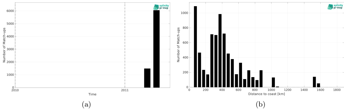
Figure 2: Number of match-ups between TSG (CSIC-UTM) and SMOS SSS L2Q v331 - With FLAG (CMEMS-CATDS-CPDC) SSS as a function of time (a) and as function of the distance to coast (b) over the South Pacific Ocean Pi-MEP region and for the full satellite product period.
