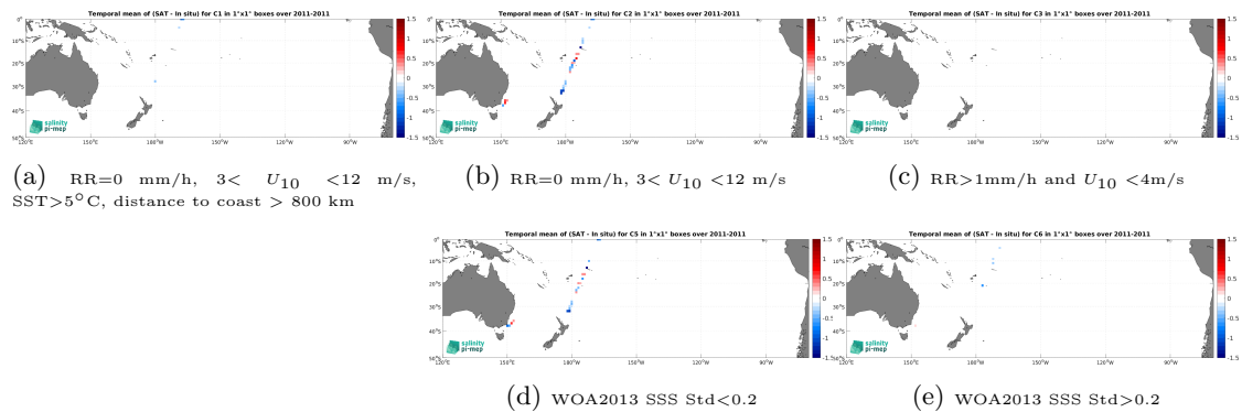
Figure 14: Temporal mean gridded over spatial boxes of size 1^\circ \times 1^\circ of \Delta SSS (SMOS SSS L2Q v331 - With FLAG (CMEMS-CATDS-CPDC) - TSG (CSIC-UTM)) for 5 different subdatasets corresponding to:RR=0 mm/h, 3 < U_{10} < 12 m/s, SST >5^\circ\text{C} , distance to coast > 800 km (a), RR=0 mm/h, 3 < U_{10} < 12 m/s (b), RR >1 mm/h and U_{10} < 4 m/s (c), WOA2013 SSS Std <0.2 (d), WOA2013 SSS Std >0.2 (e).
