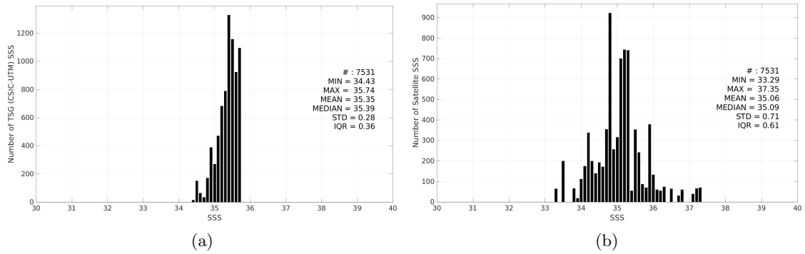
Figure 3: Histograms of SSS from TSG (CSIC-UTM) (a) and SMOS SSS L2Q v331 - With FLAG (CMEMS-CATDS-CPDC) (b) considering all match-up pairs per bins of 0.1 over the South Pacific Ocean Pi-MEP region and for the full satellite product period.
